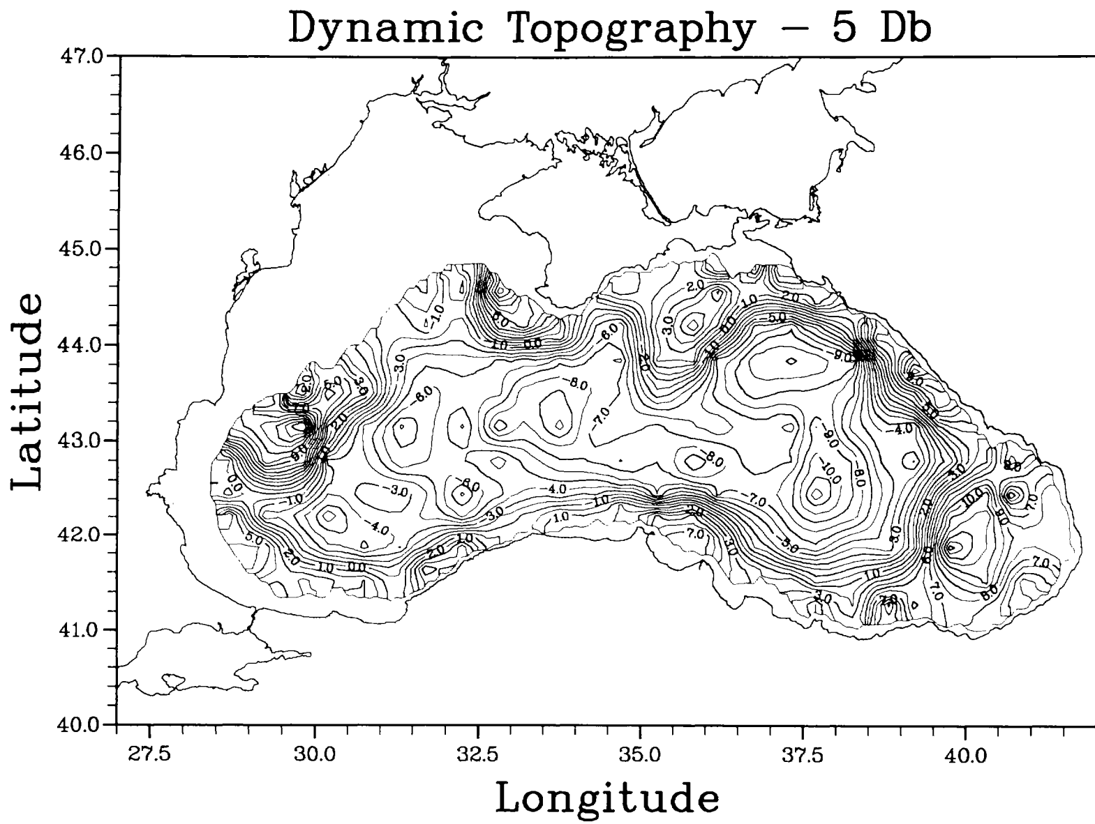
Figure 36: Dynamic topography for stations having depths exceeding 900 m. The dynamic topography is for 5 db level, referenced to 900 db.
