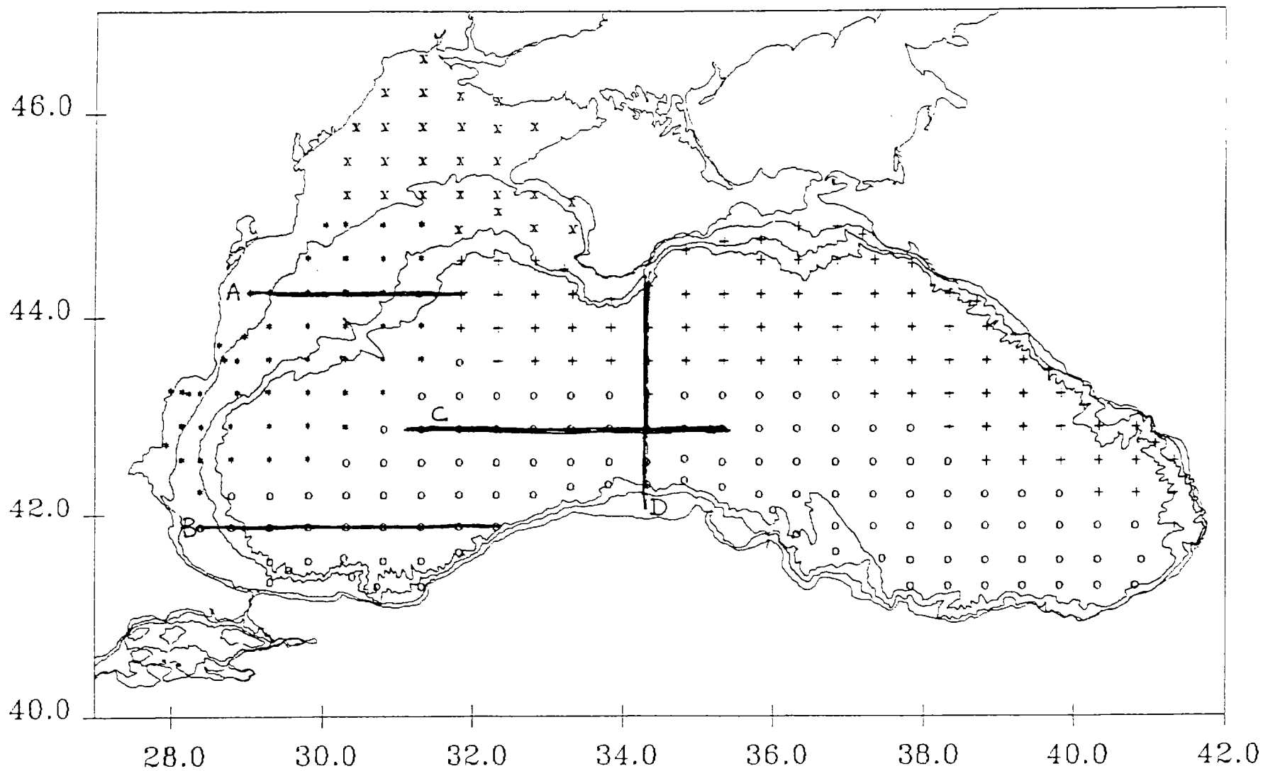
Figure 1. Station locations for HydroBlack '91. Circles are Turkish stations, asterisks are Romanian and Bulgarian stations, crosses and x's are Ukrainian and Russian stations.
