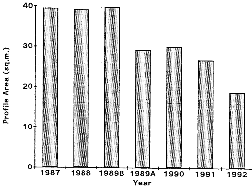
FIGURE 47 Pagua Bay Annual Changes 1987-1992
