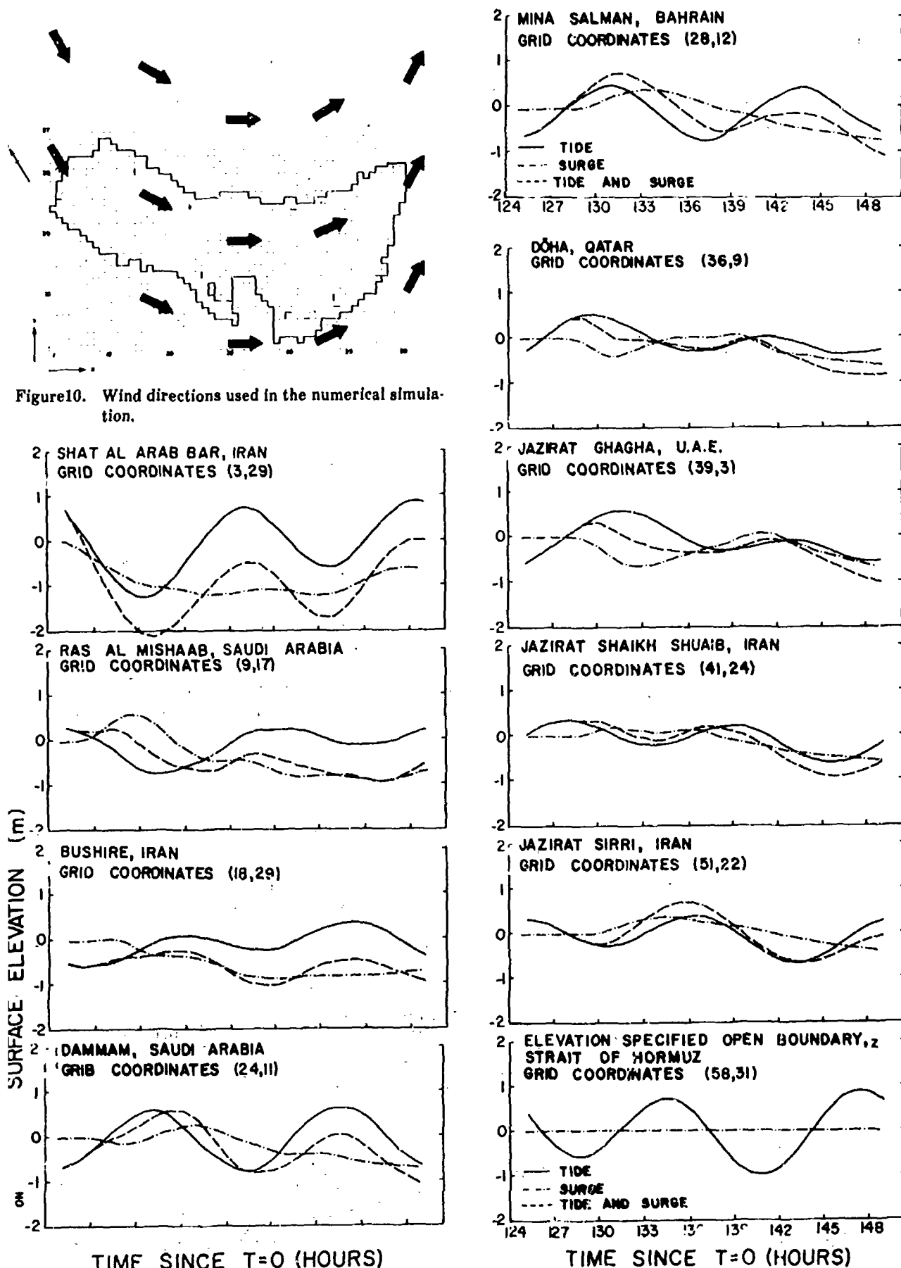
Figure 11. Computed profiles of the tide (six constituents M_2 , S_2 , N_2 , K_1 , O_1 , P_1 are included), surge plus tide and surge only at selected locations.
