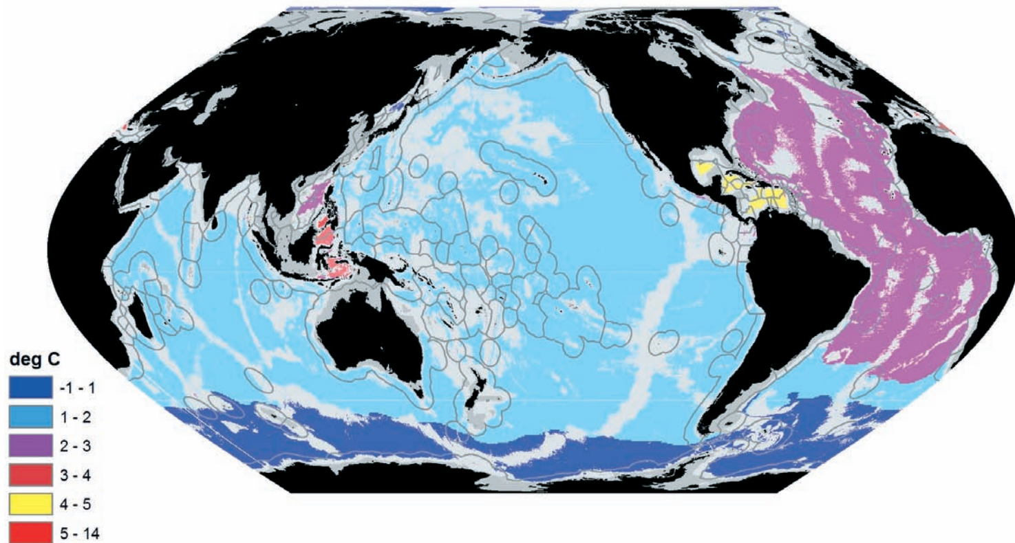
FIGURE 16: Annualized bottom water temperature at 3500 m, with depths 3500 – 5500 m visible.
