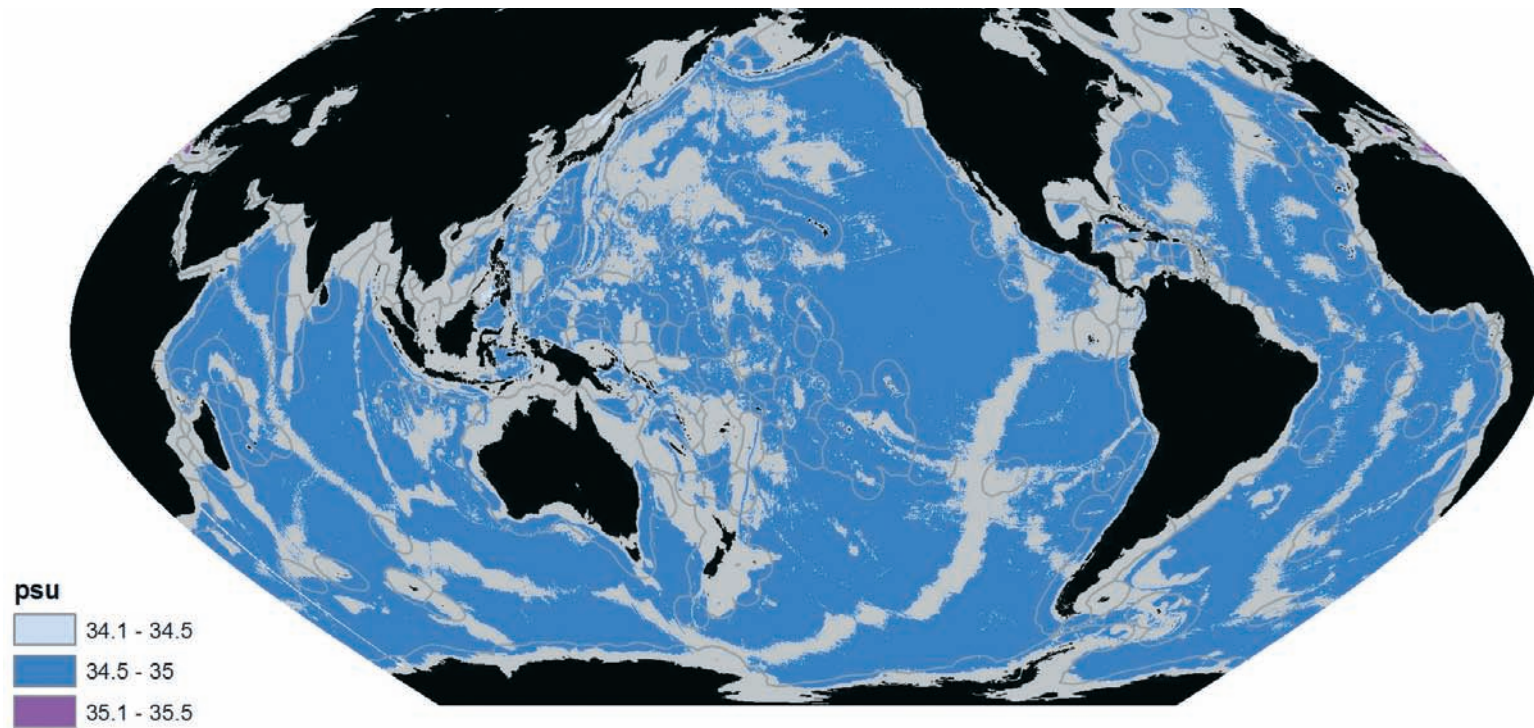
FIGURE 20: Annualized bottom water salinity at 3500 m, with 3500 – 5500 m depth interval visible.
