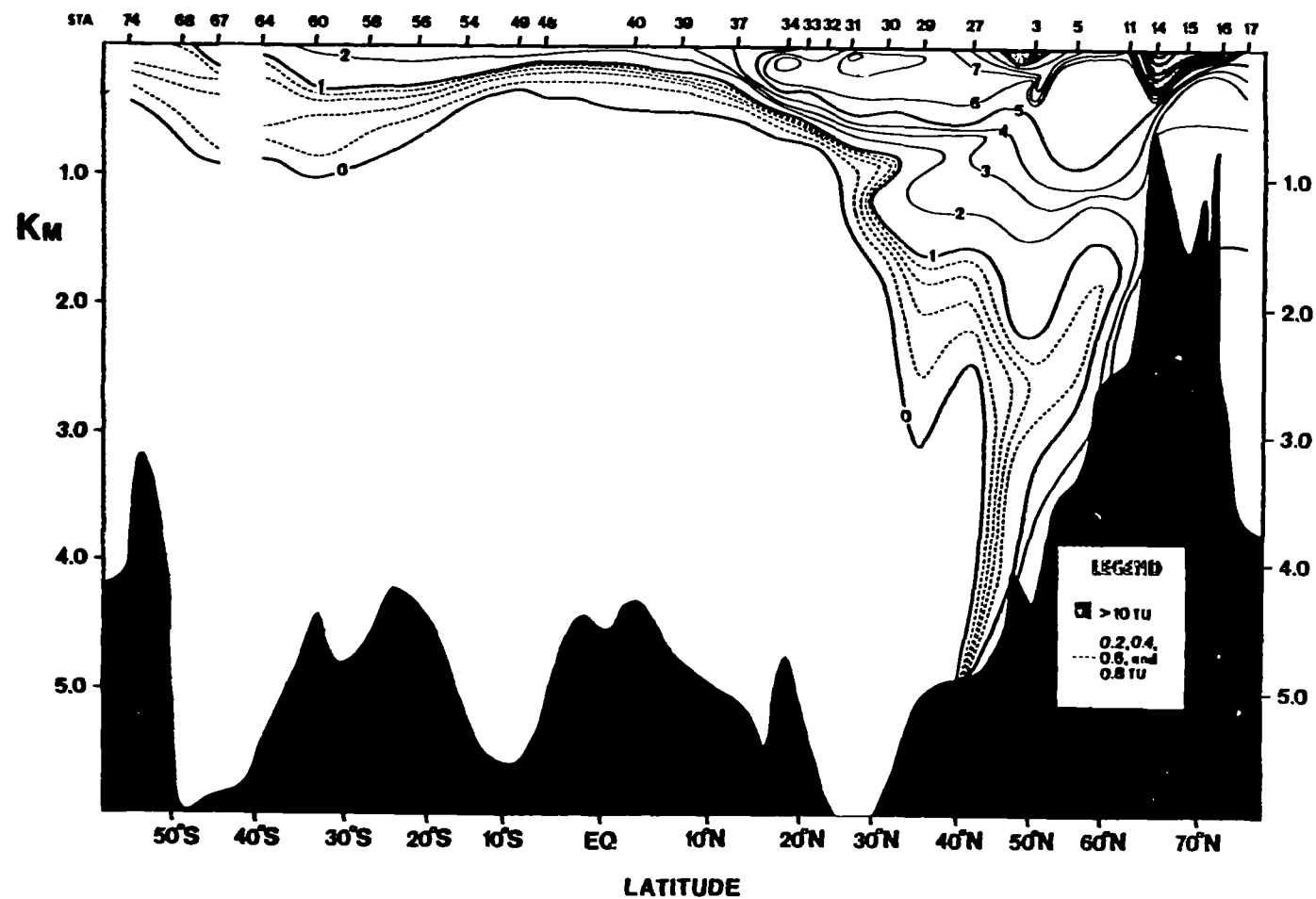
Figure II.2 : Western Atlantic tritium during GEOSecs taken from Ostlund et al. (1976)
