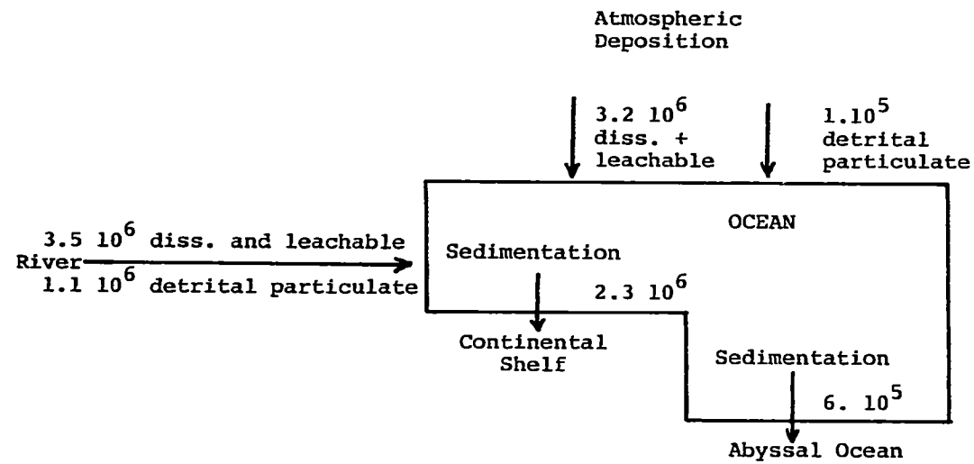
Figure III.3 : Fluxes of cadmium through the marine environment (from ICES 1982)
