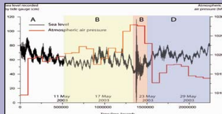
Spectral and temporal wave-by-wave analysis of tsunami waves measured in the near-shore zone of Palma de Majorca and Sant Antoni (Spain) caused by the 2003 Zemmouri (Boumerdès) earthquake (Mw=6.9), Algeria.
