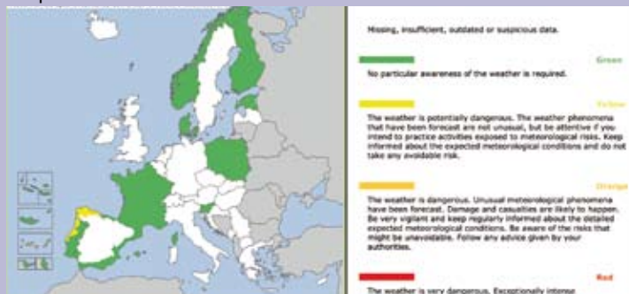
Example of coastal event for Europe on 30th October 2011 at 18:02
