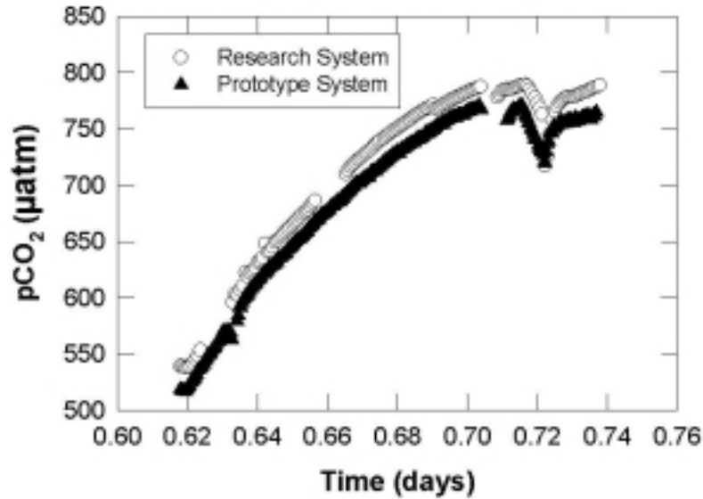
Figure 8. Bench top comparison of the two systems
