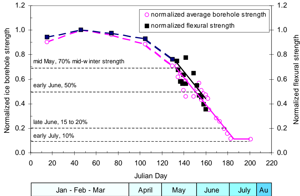
• Figure 7: Comparison of normalized ice borehole strength and calculated flexural strength
