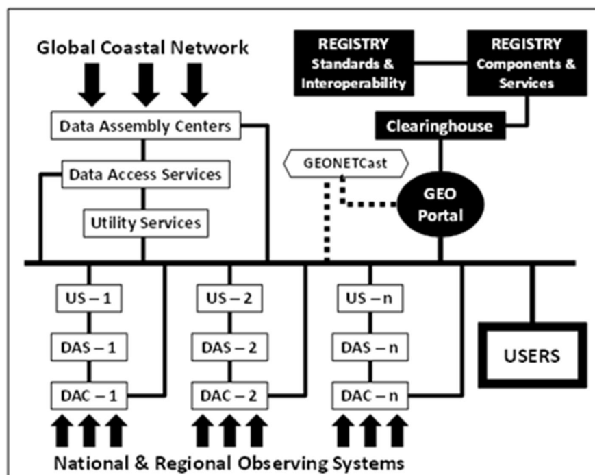
Figure 24. Service-Oriented Architecture for coastal GOOS (white boxes: US – Utility Services, DAS – Data Access Services, DAC – Data Assembly Centers) with linkages to the GEOSS Common Infrastructure (black compartments). Data dissemination and access are via the internet (thick horizontal line) and satellite-based communications systems (dashed line).
