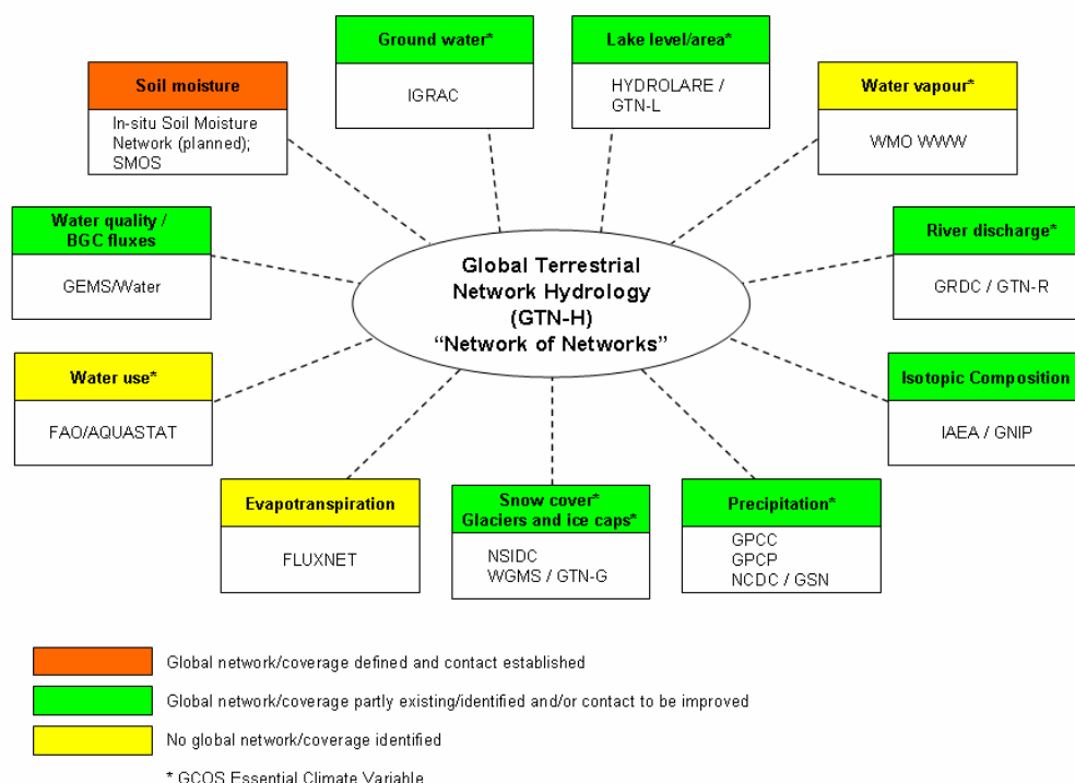
Figure 23: Configuration of the Global Terrestrial Network for Hydrology (GTN-H) (April 2009).
