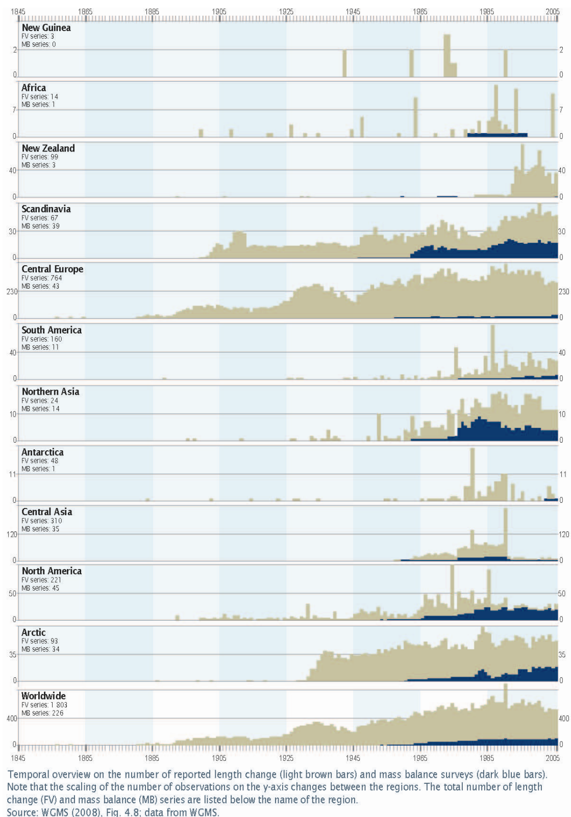
Figure 26 Glacier length change and mass balance surveys contributing to the Global Terrestrial Network Glaciers (GTN-G) (Source: WGMS).
