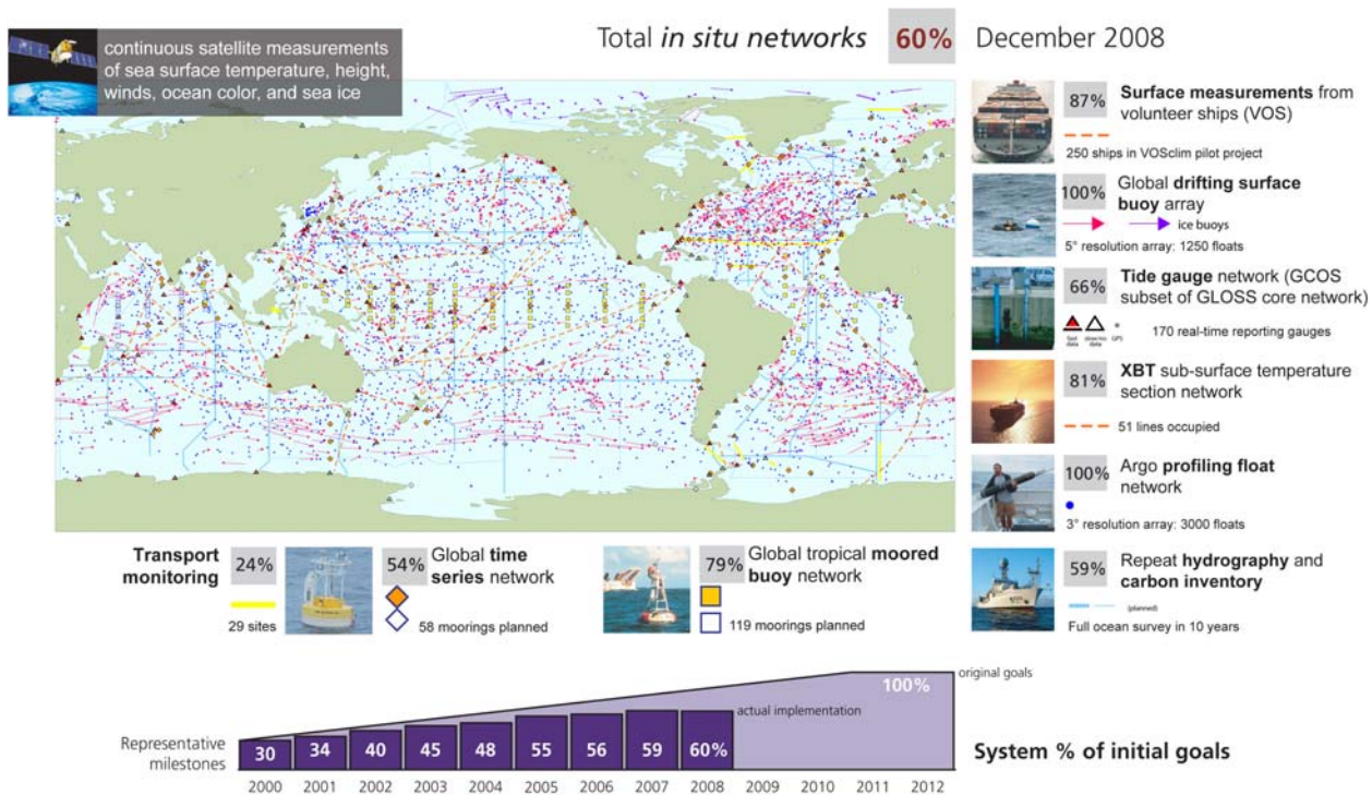
Figure 15: Status of the in situ global ocean observing system. By December 2008, total implementation reached 60% of its initial goals. Note that gaps between individual systems are significant despite the overall impression of dense in situ coverage of the oceans. Implementation has progressed steadily but slowly, falling short of the original goals.
