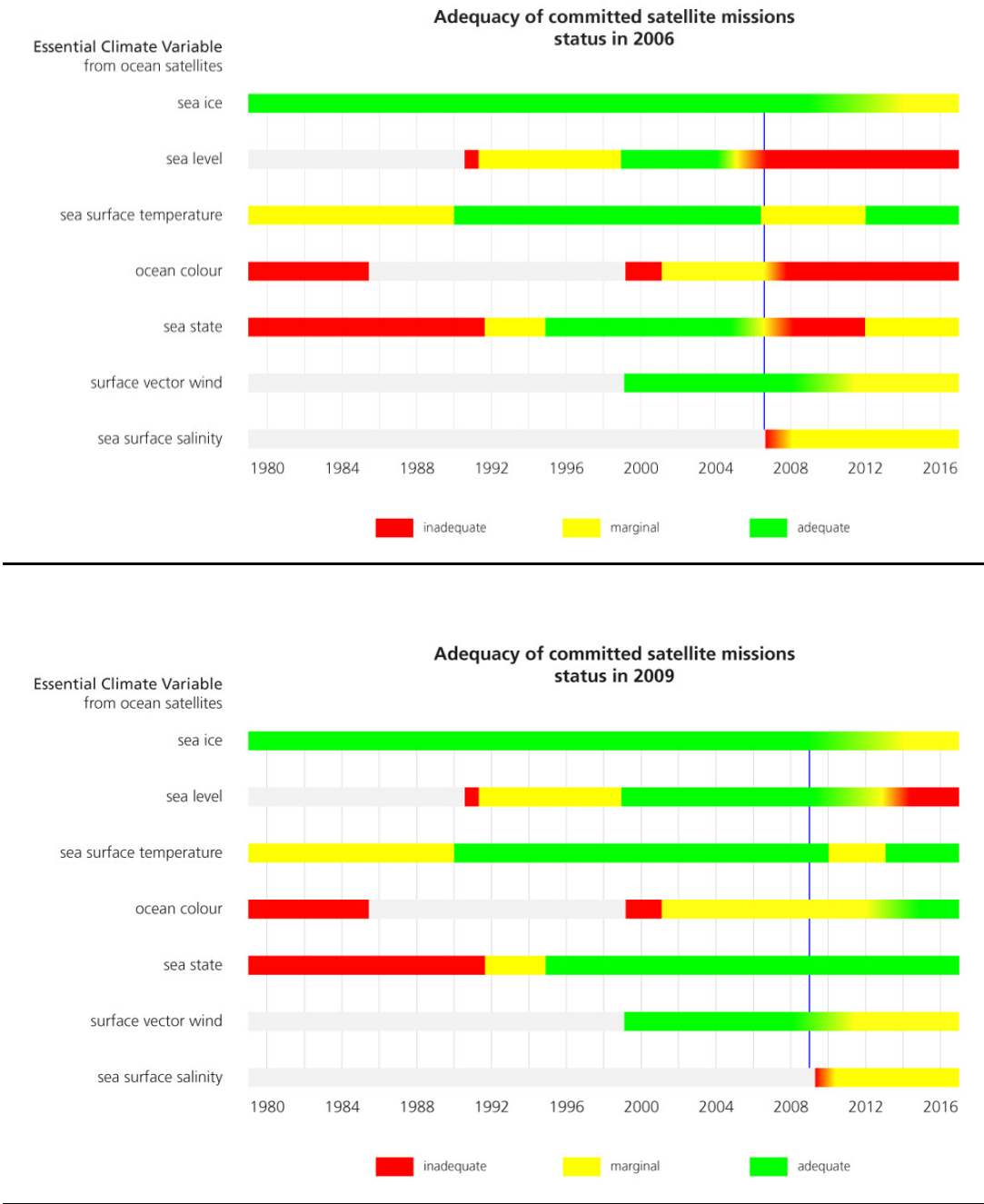
Figure 17: Improvement in the commitments by satellite agencies to continuous climate-quality measurements of sea-surface ECVs by satellite has been substantial since 2006 (top, 2009 in bottom figure). The colour bars indicate the adequacy of committed satellite missions by the research and operational space agencies for the requirements set in IP-04 and the Satellite Supplement. Marginal adequacy meets the requirements but relies on missions that are past their planned lifetime or with no redundancy.
