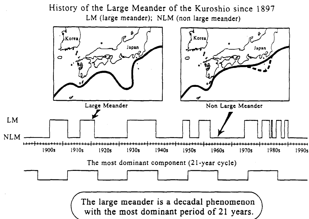
Figure 2. History of the large meander of the Kuroshio during one century since 1897 and its dominant cycle.
