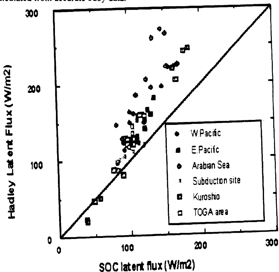
Figure 8.1-2 Comparison of SOC latent heat flux values computed with corrected VOS data vs. flux values produced by the Hadley model showing model bias.
