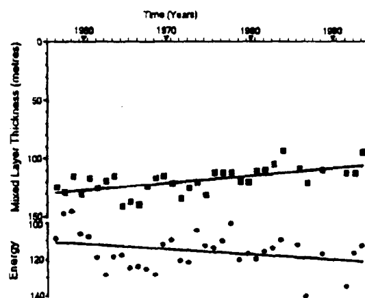
Figure 4: Mixed layer characteristics at Station Papa, 1956 to present.
