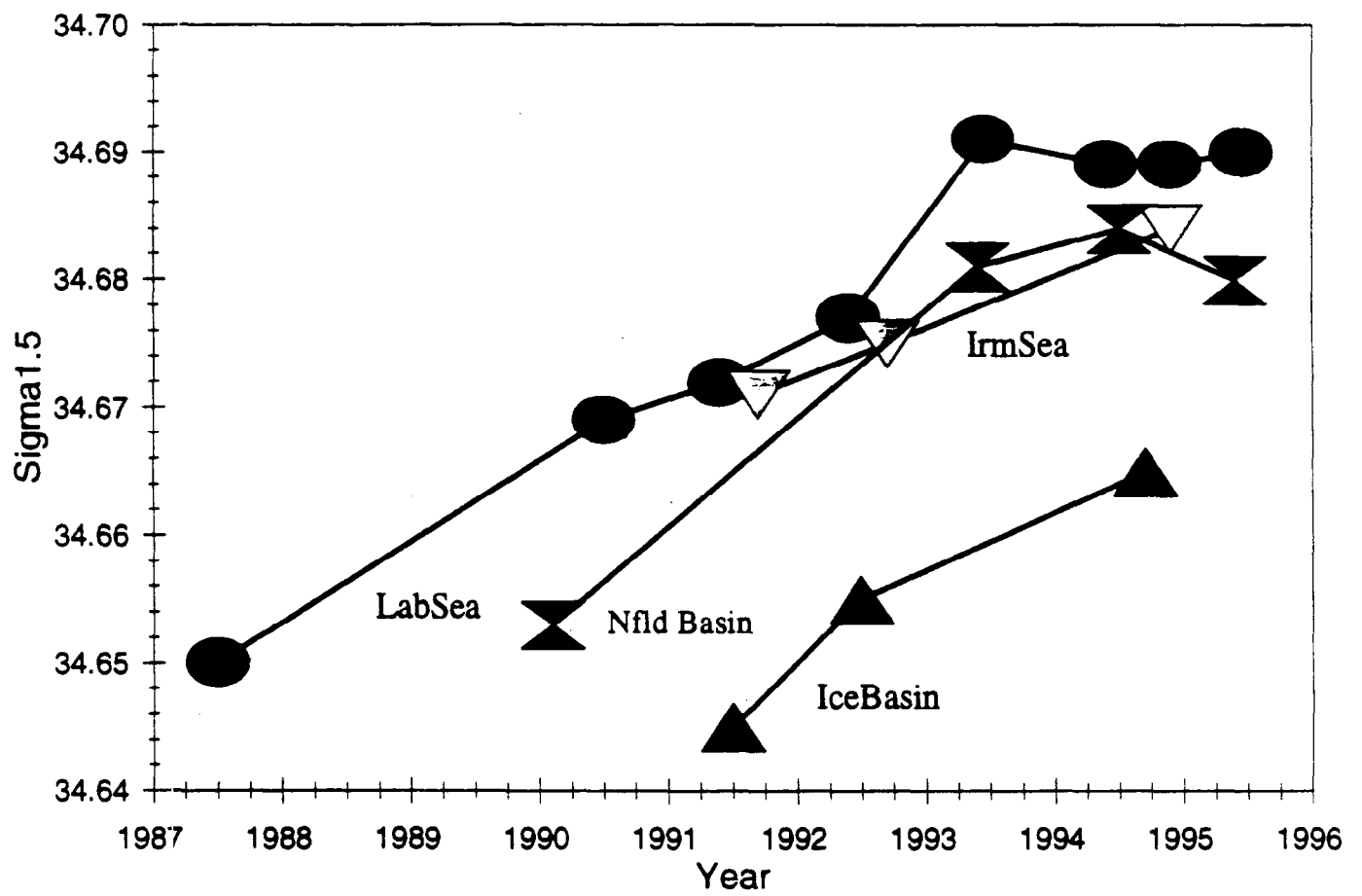
Fig.14. Potential density anomaly referenced to 1500 db (sigma1.5) at the core of the Labrador Sea Water for the years, locations and sources cited in Fig. 13.
