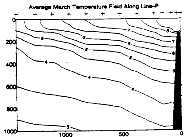
Figure 2: Mean March temperature along Line-P
