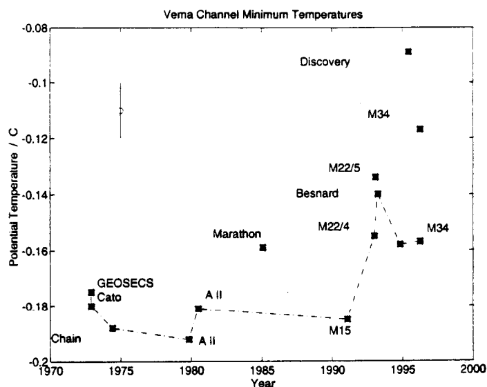
Figure 4.6-1. Time-series of potential temperatures from the bottom of the Vema Channel. This over 4.6 km deep conduit enables equatorward spreading of Antarctic Bottom Water after its passage through the Argentine Basin to enter the Brazil Basin. Only those values that could be located in the cold Weddell Sea Deep Water, the lowest part of Antarctic Bottom Water, were connected by line segments. The given error bar at year 1975 represents a conservative estimate that has decreased with the advent of high-precision CTD instruments during the course of the time-series. For a detailed discussion see Zenk and Hogg (1996) and Hogg and Zenk (1997).
