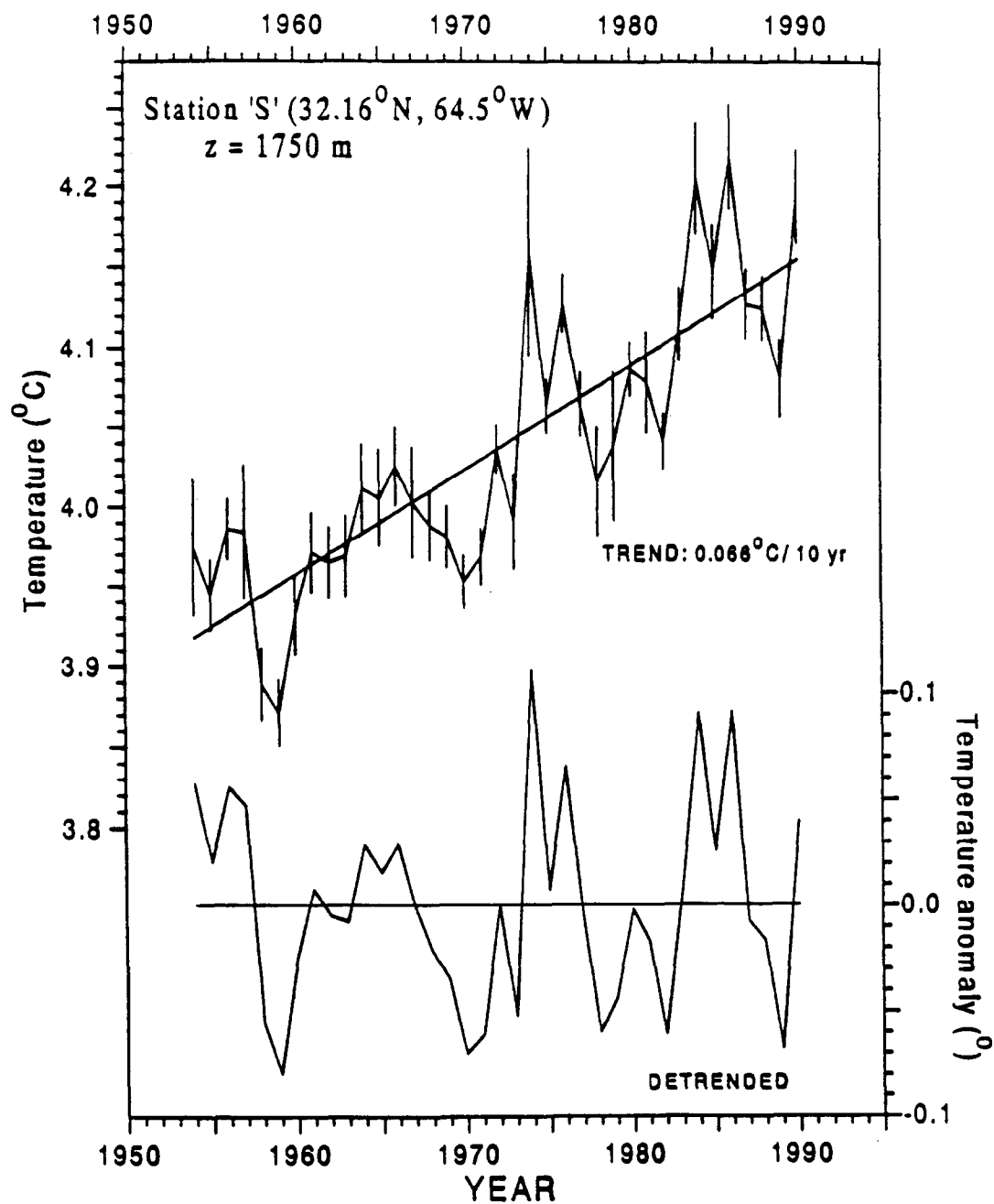
Fig. 1. Time series of yearly mean temperatures at 1750 depth at Station "S" located in the subtropical gyre of the North Atlantic Ocean near Bermuda. The yearly means are computed from the average of the twelve monthly means in each year. The vertical bars extending from each yearly mean represent plus and minus one standard error of the twelve monthly means about each yearly mean. The bottom half of the figure has the linear trend removed.
