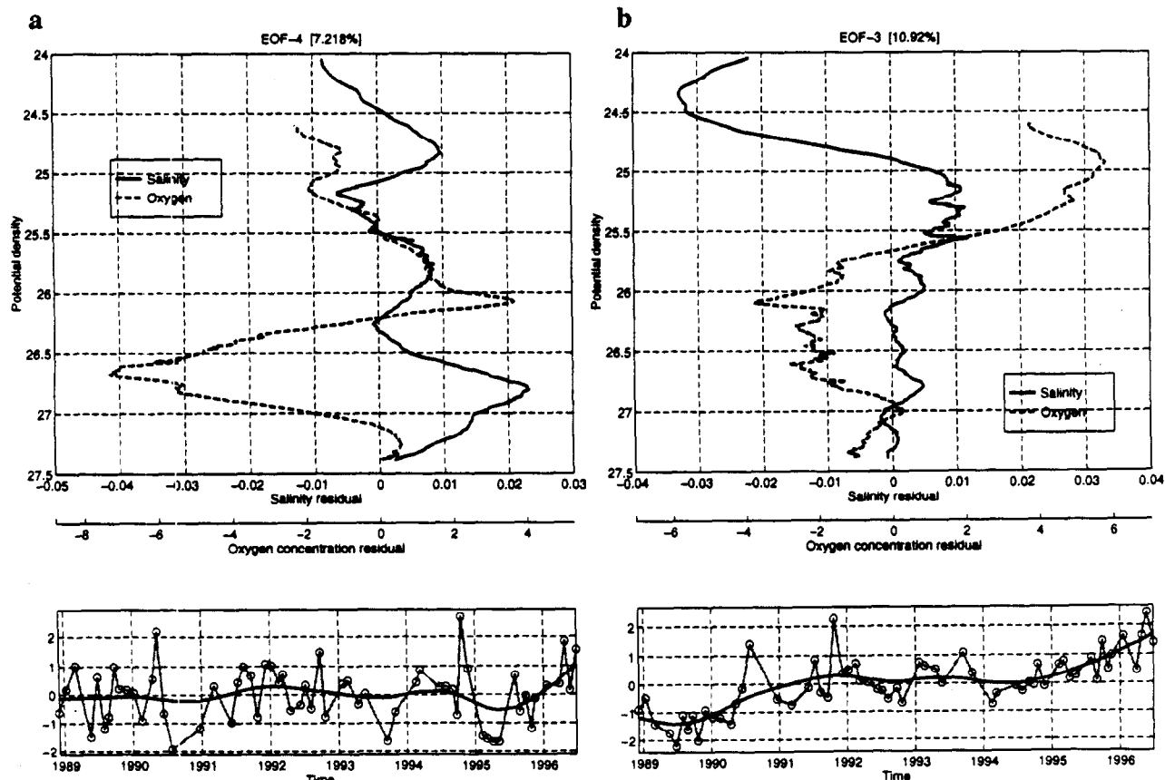
Figure 6. Joint EOF analysis of salinity and dissolved oxygen ( \mu \text{mol/kg} ) residuals on potential density surfaces. The mean, annual, and semiannual signals were removed from the data prior to the analysis. The 4th (a), and 3rd (b) EOFs versus \sigma_{\theta} are shown in the upper panel, and the lower panel shows the time series.
