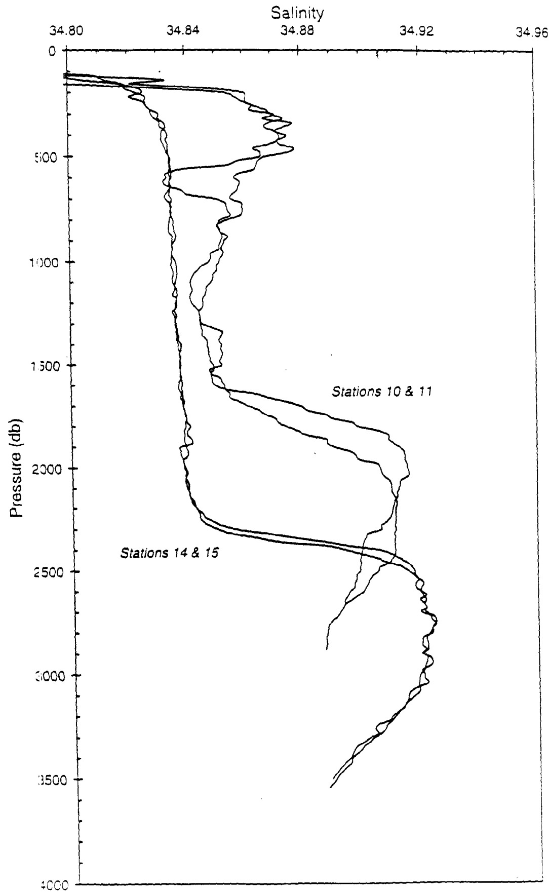
Fig.4. Vertical profiles of salinity obtained in June 1993 in the central Labrador Sea and over the continental slope.
