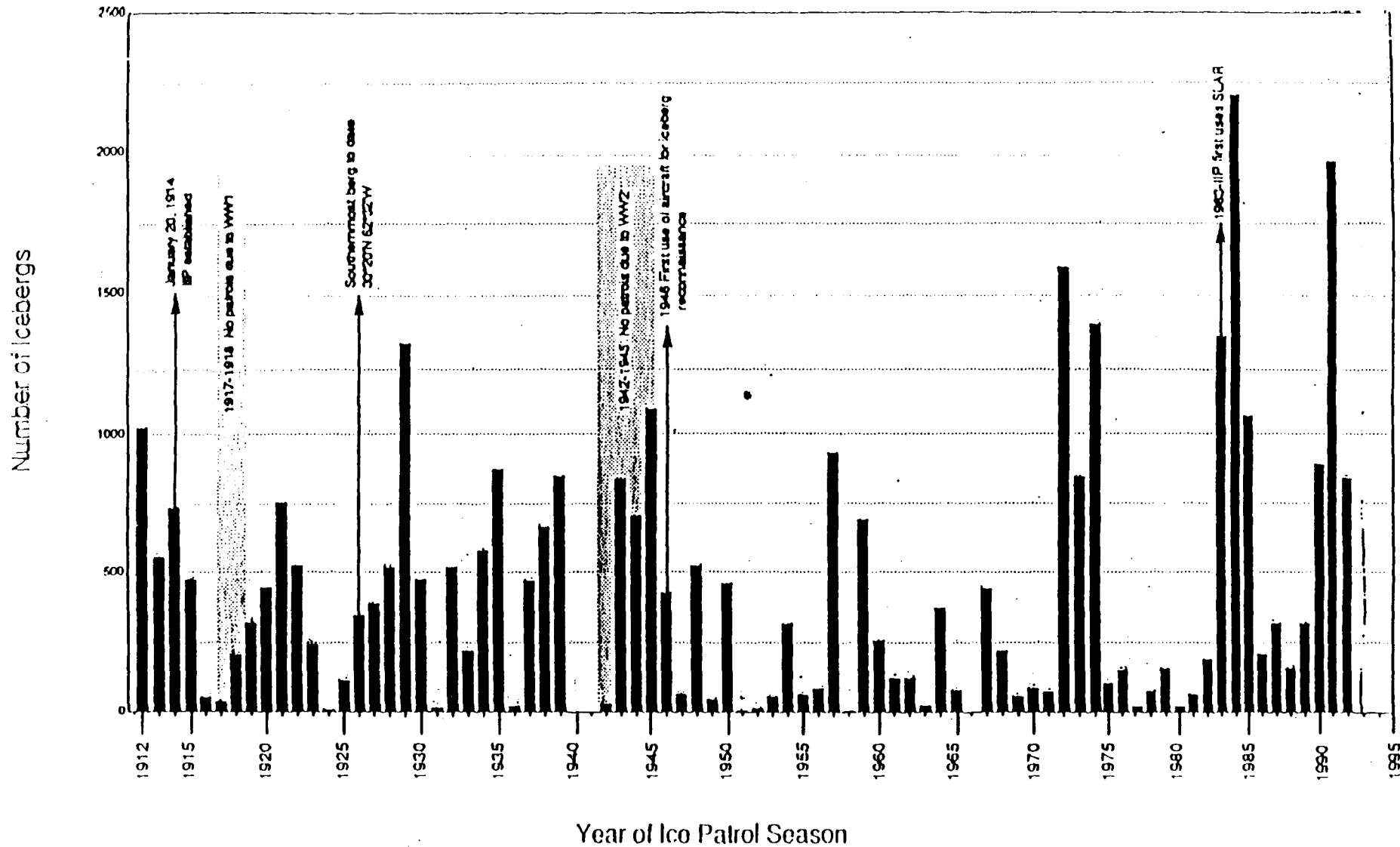
Fig.5. Number of icebergs moving south in the Labrador Current past 48° N between 1912 and 1992, (Pers. Comm. Donald Murphy, USCG)
