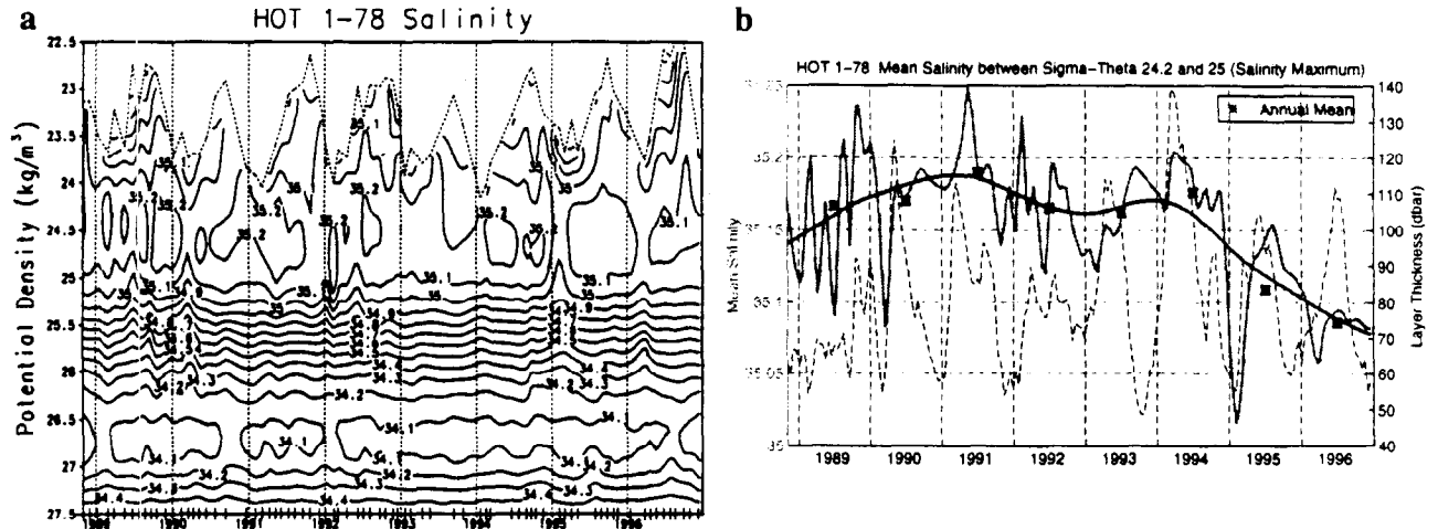
Figure 3. a) Contours of salinity measured by CTD versus \sigma_\theta for HOT cruises 1 to 78. The average density of the sea surface for each cruise is connected by a dashed line. Data are the average of all casts for each cruise. b) Time-series of mean salinity (gray solid line) between the 24.2 \sigma_\theta and 25.0 \sigma_\theta isopycnals. The smooth line is a spline fit to the data. The asterisks show the annual mean. The dashed line is the thickness of the layer between the two isopycnals.
