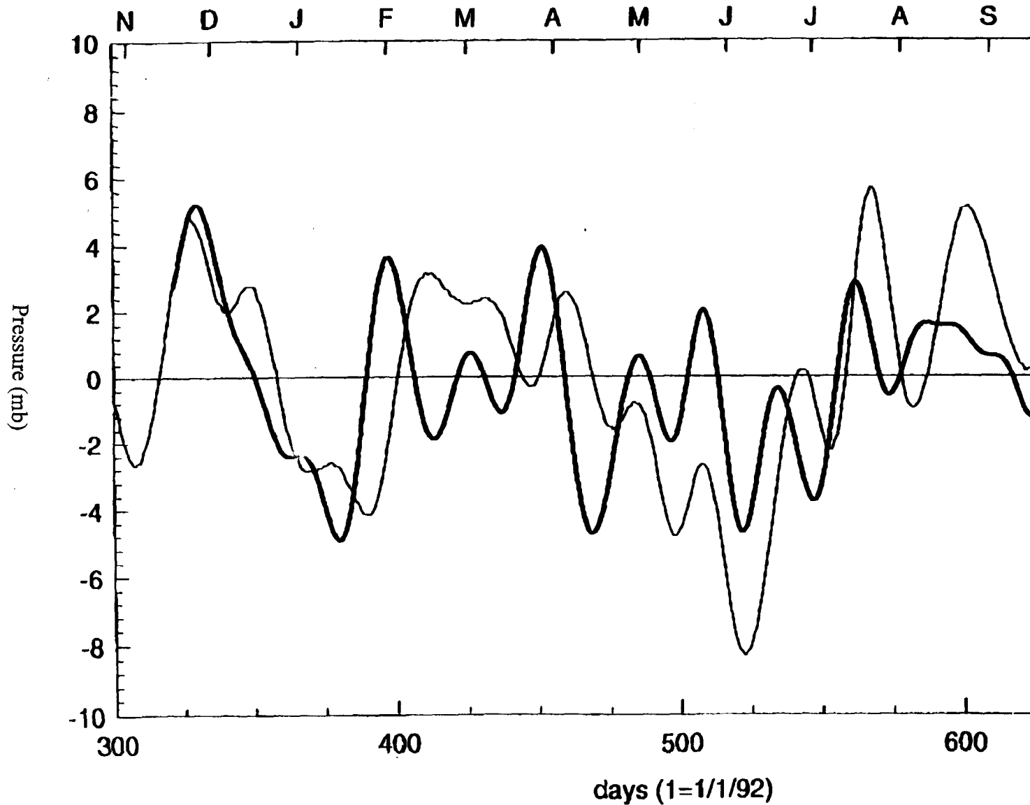
Figure A-2. Pressure difference at Drake Passage (north minus south; heavy line) and between Africa and Antarctica (SANA-E) for the period of concurrent operation. The series have been smoothed with a 21-day filter. The y-axis scale is in mb. The x-axis scale is in days (1=1/1/92).
