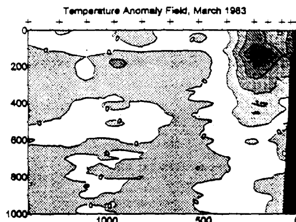
Figure 3: The temperature anomaly field for March 1983.
