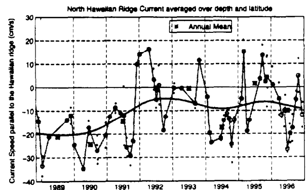
Figure 4. Magnitude of the current (dots) measured with an ADCP during HOT cruises, averaged between 20 and 110 m and between 21.7°N and 22.6°N. The circles are the averages per cruise, and the smooth line is a cubic spline fit to the averages. The asterisks show the annual mean.
