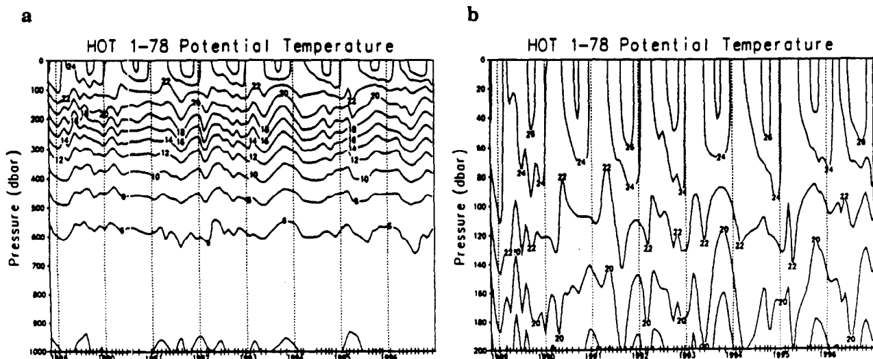
Figure 1. Contours of potential temperature (°C) measured by CTD versus pressure in the upper 1000 (a) and 200 (b) dbar for HOT cruises 1-78. Cruise times are indicated by the tick marks along the bottom axis. Data are the average of all casts for each cruise.
