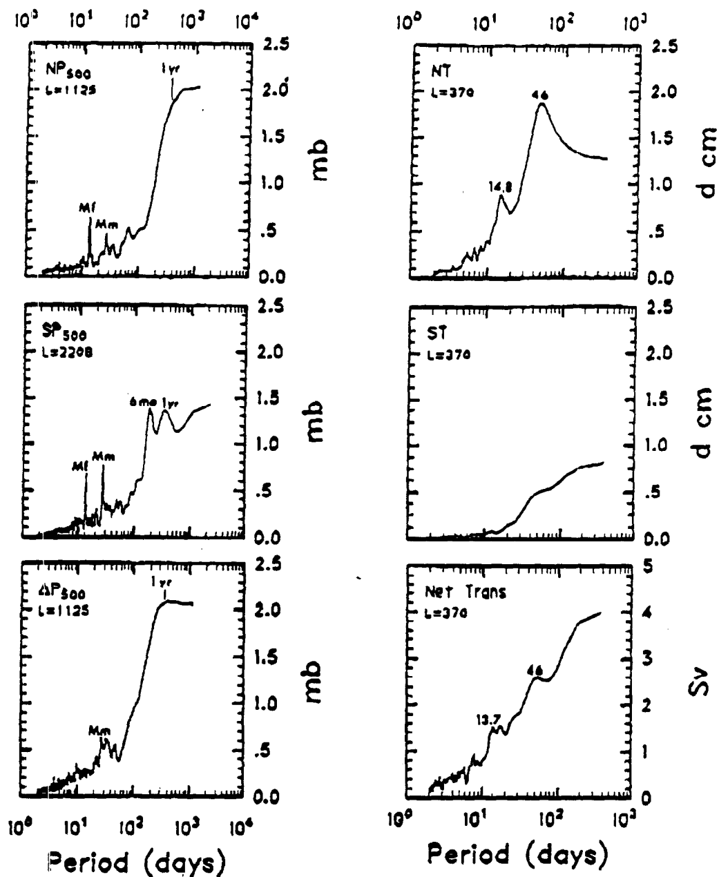
Figure 2. Time series of autospectra of 500-m pressure and geopotential anomaly at the northern (Npand NT) and southern (SP and ST) sides of Drake Passage nad of the difference ( \Delta P_{500} ) and net transport; seasonal to annual peaks are evident.
