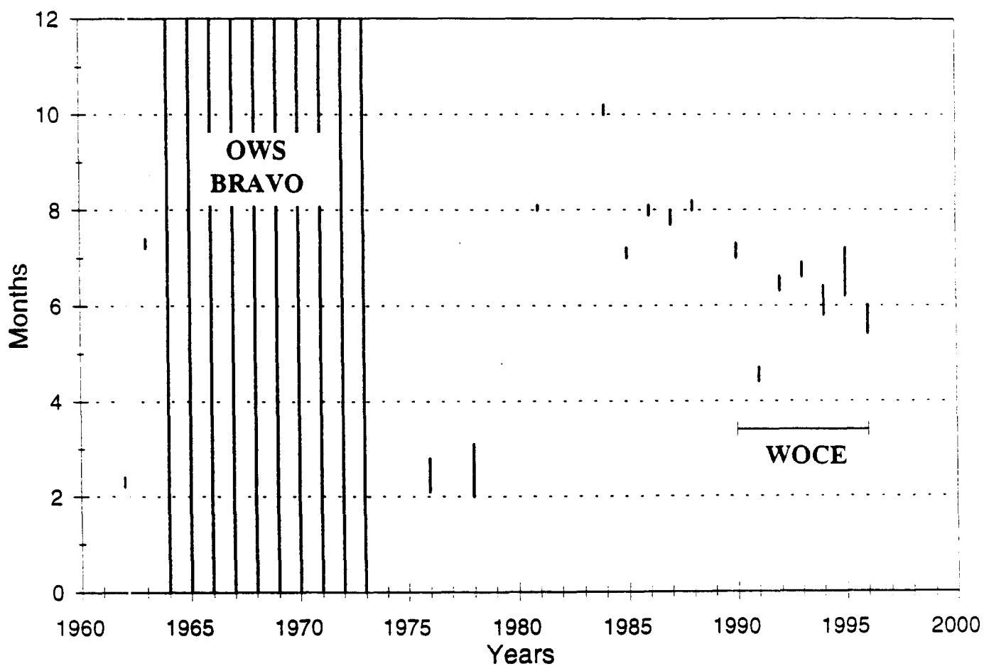
Fig.2 Times of deep oceanographic measurements in the central Labrador Sea between 1962 and 1996 including those from the OWS Bravo and the WOCE AR7W line across the Labrador Sea.
