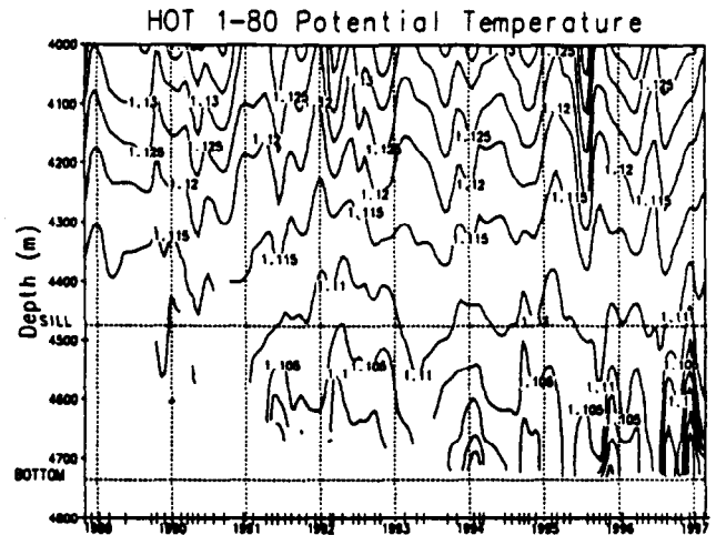
Figure 9. Same as Figure 8a, except versus depth below 4000 m for cruises 1-80. Horizontal lines indicate the depth of the sill (see text) and bottom.
