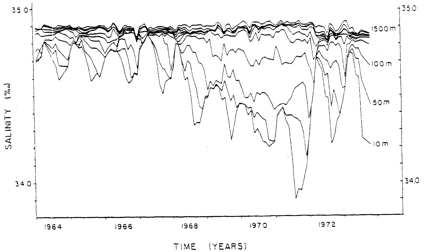
Fig.8. Monthly averages of salinity at eleven depths at station Bravo from 1964 to 1973 from Lazier (1980).
