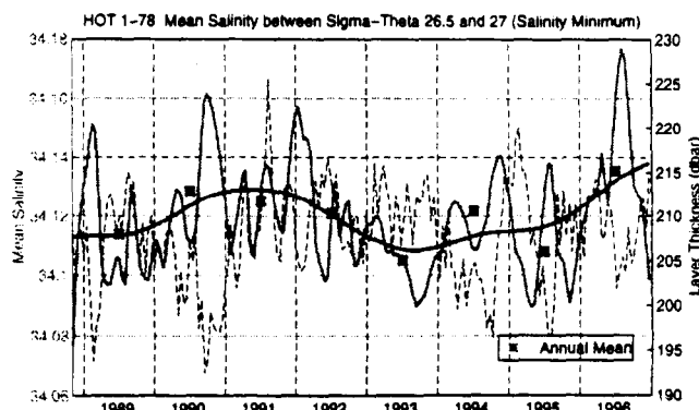
Figure 5. Same as Figure 3b, except for Salinity between 26.5 \sigma_{\theta} and 27 \sigma_{\theta} isopycnals.
