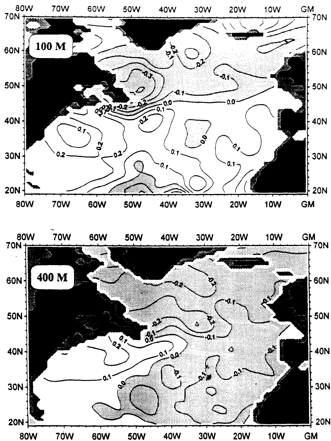
Fig. 3 Linear temperature trend ( ^{\circ}\text{C}/10 years) at 100 and 400 m depth in the North Atlantic Ocean.
