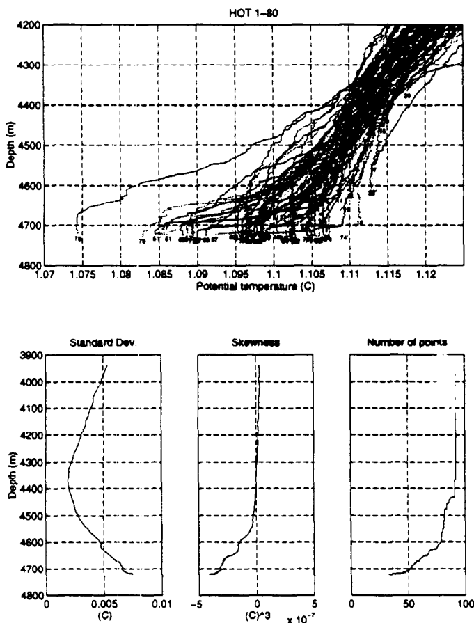
Figure 9. Same as Figure 8a, except versus depth below 4000 m for cruises 1-80. Horizontal lines indicate the depth of the sill (see text) and bottom.
