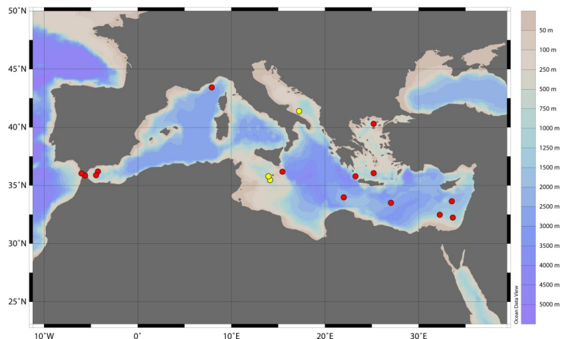
Figure 4: locations of all the Mediterranean stations with \epsilon\text{Nd} data (red circles: stations with published values; yellow circles: cruises Medcor in the Siculo-Tunisian Strait and Arcadia in the Adriatic Sea; Montagna et al., unpublished data).
