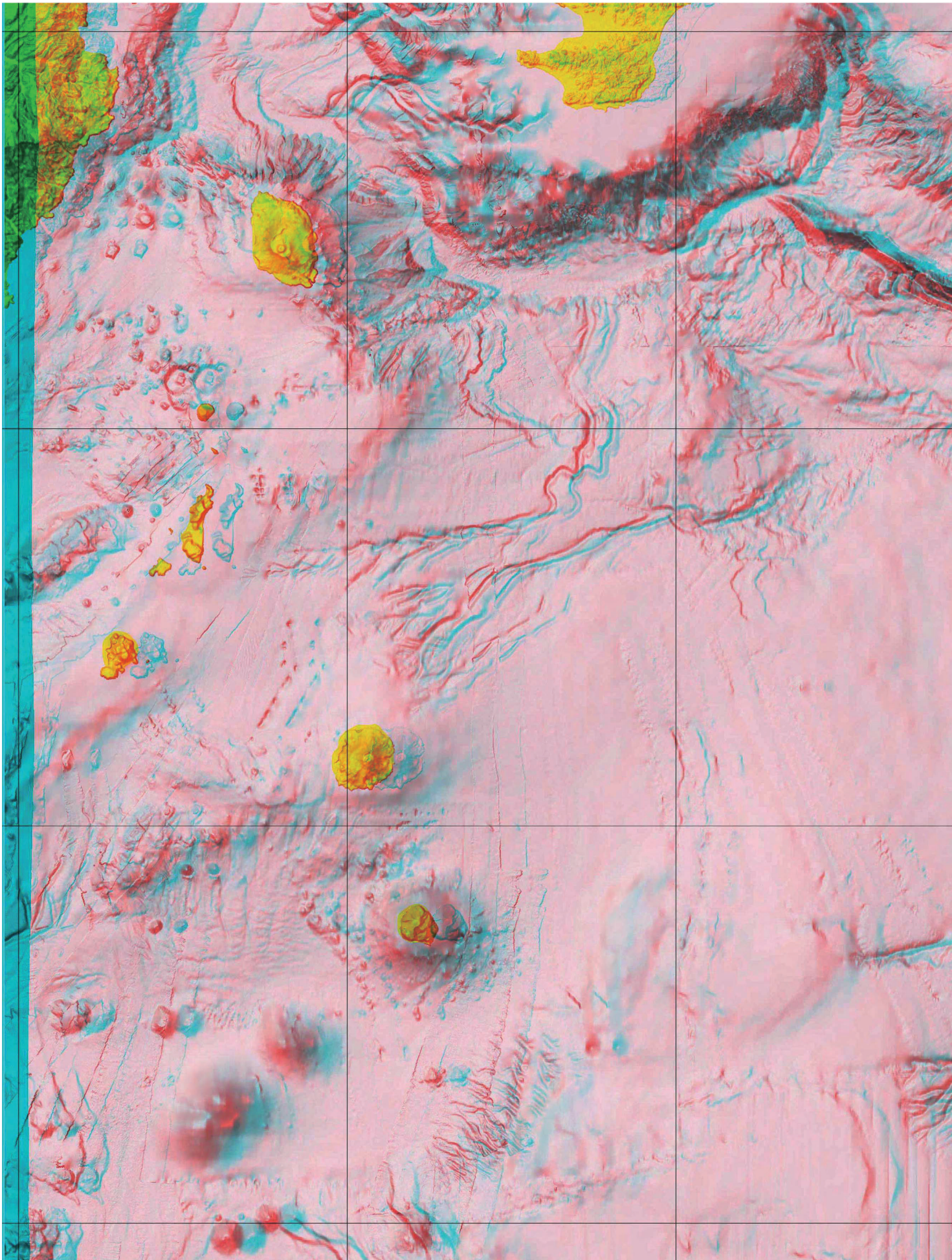
Fig. 6 Anaglyph image of the Sagami Trough and the Boso Triple Junction.
