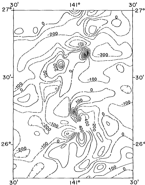
Fig. 46 Geomagnetic total intensity anomaly chart of Kaikata and Kaitoku Seamount surveyed in 1985 and 1986. Contour interval 100nT.
