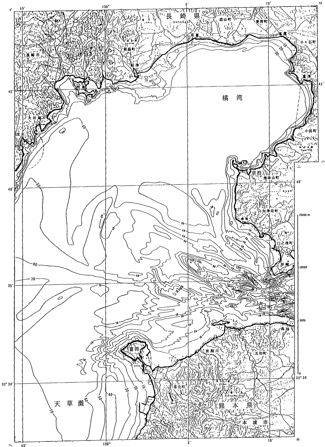
Fig. 4 Topography of Tatibana Bay surveyed in 1993.
