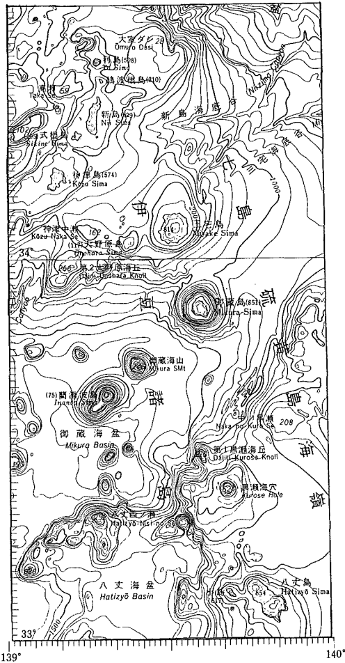
Fig. 28 Topography of Izu Shoto sea area, Omuro Dasi to Hatizyo Sima (after chart No.6313).
