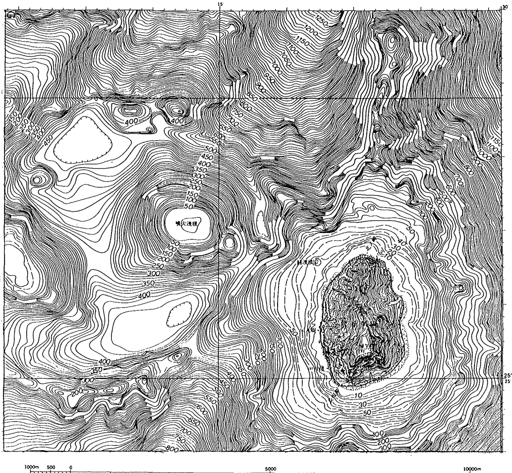
Fig. 48 Topography around Kita-Io Sima surveyed in 1992. Contour interval 10m.
