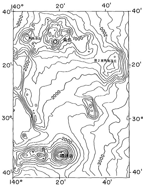
Fig. 39 Topography around Tori Sima and Sofu Gan surveyed in 1986. Contour interval 200m.
