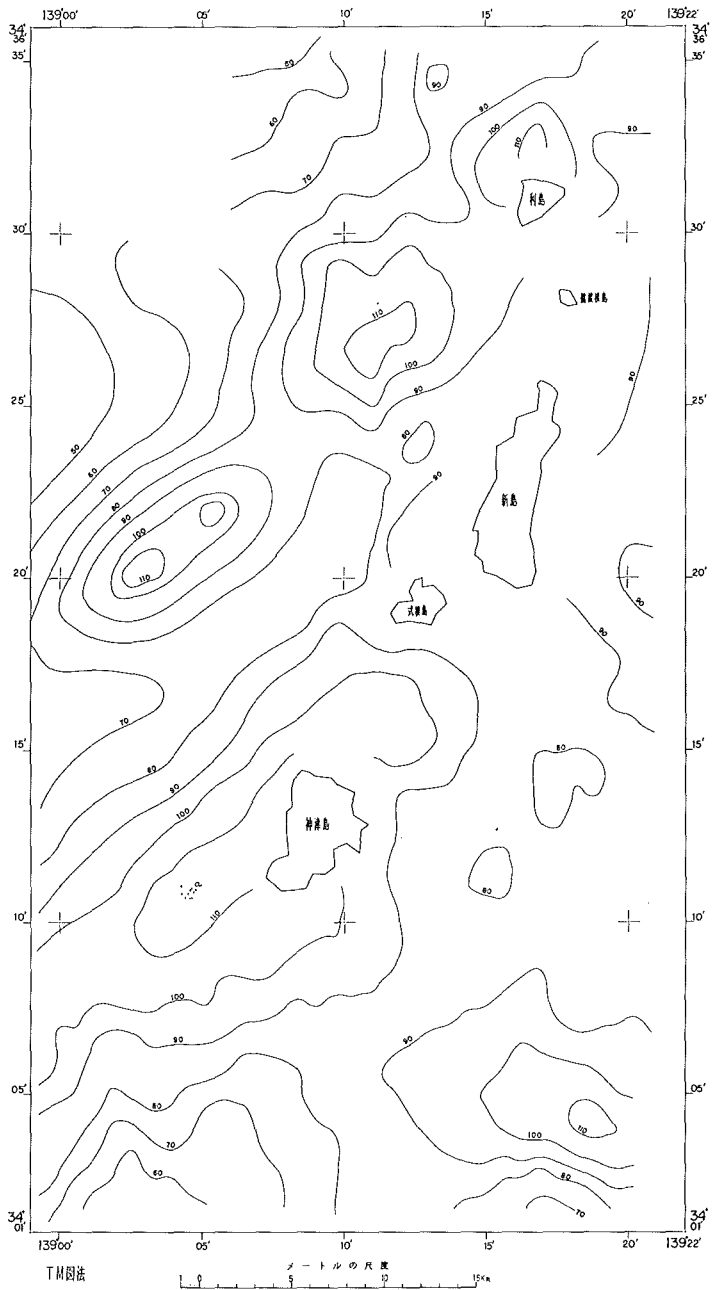
Fig. 27 Free air Gravity anomaly chart around Nii Sima and Kozu Sima surveyed in 1993. Contour interval 10mGal.
