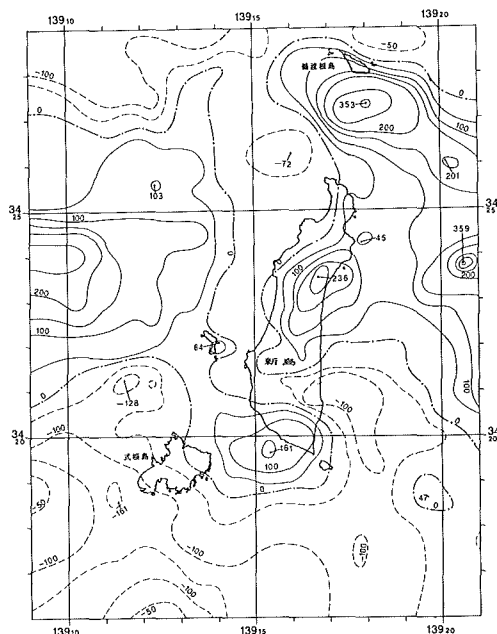
Fig. 24 Aeromagnetic total intensity anomaly chart over Nii Sima from Report of Coordinating Committee for Prediction of Volcanic Eruption , No.44. (1989) Contour interval 50nT.
