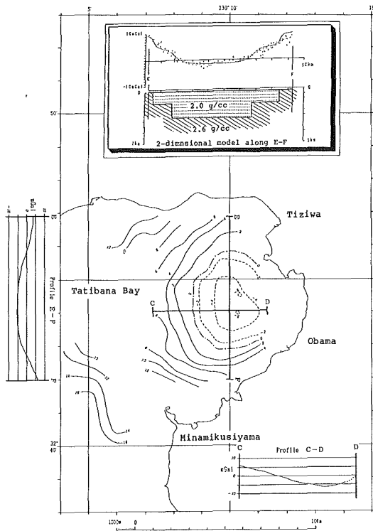
Fig. 6 Free air gravity anomaly chart in Tatibana Bay after Hydrog. Dep. Survey Team(1992).
