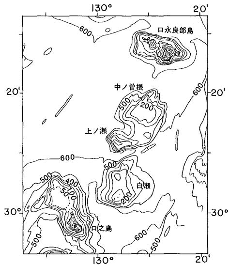
Fig. 10 Topography from Kutinoerabu Sima to Kuti-no-Sima surveyed in 1974 and 1981. Contour interval 100m.
