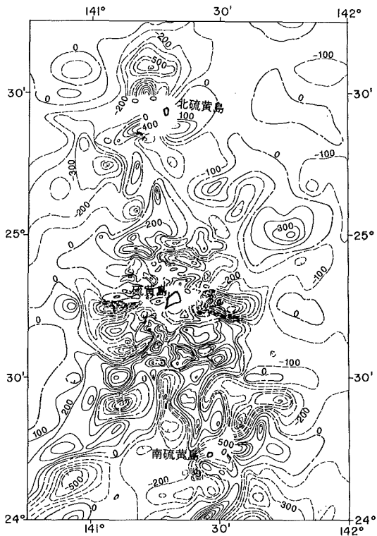
Fig. 50 Geomagnetic total intensity anomaly chart from Kita-Io Sima to Minami-Io Sima surveyed in 1981, 1985 and 1986. Contour interval 100 nT.
