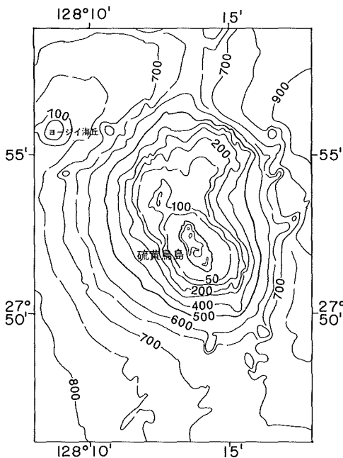
Fig. 13 Topography of Io-Tori Sima Volcano surveyed in 1986. Contour interval 100m.
