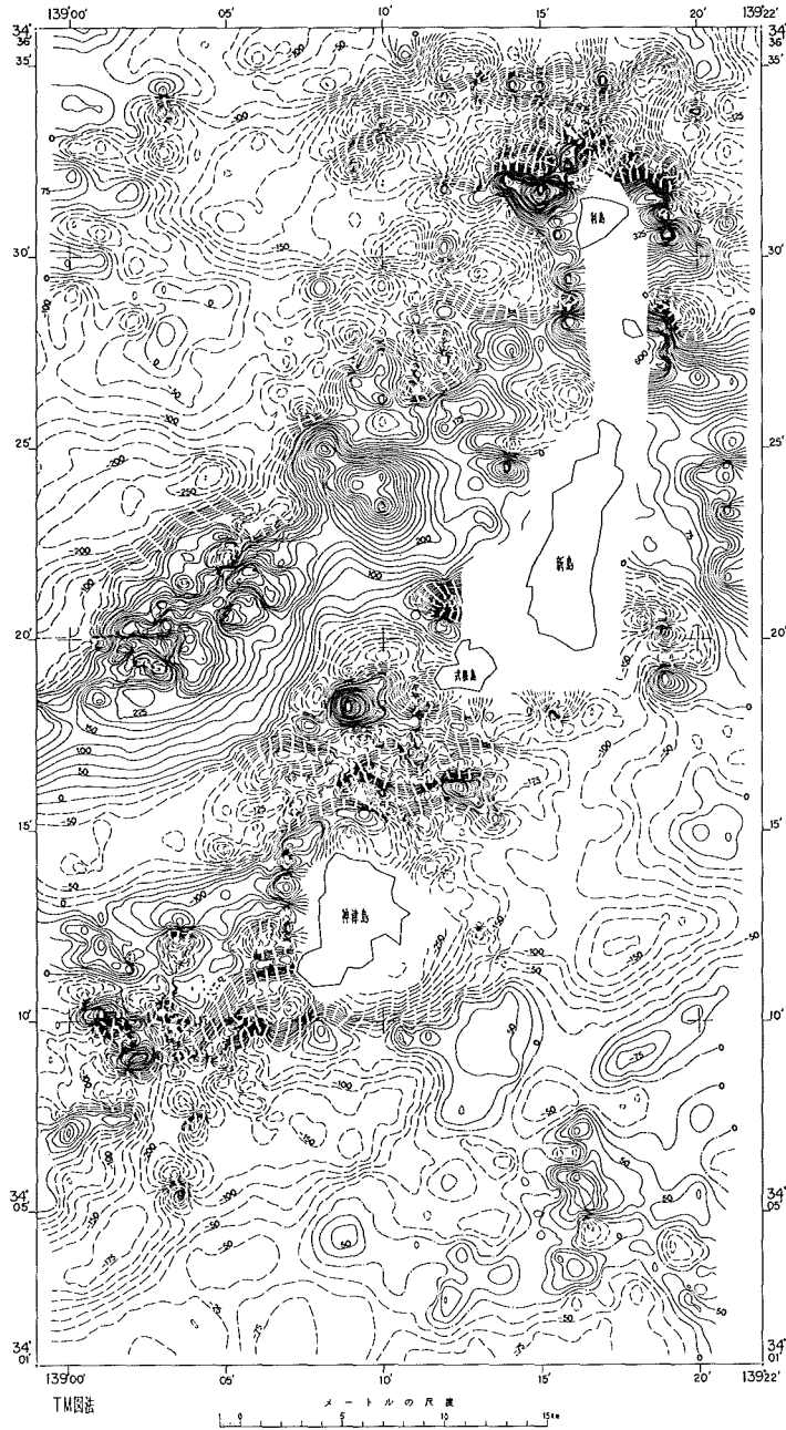
Fig. 26 Geomagnetic total intensity anomaly chart around Nii Sima and Kozu Sima surveyed in 1993. Contour interval 25nT.
