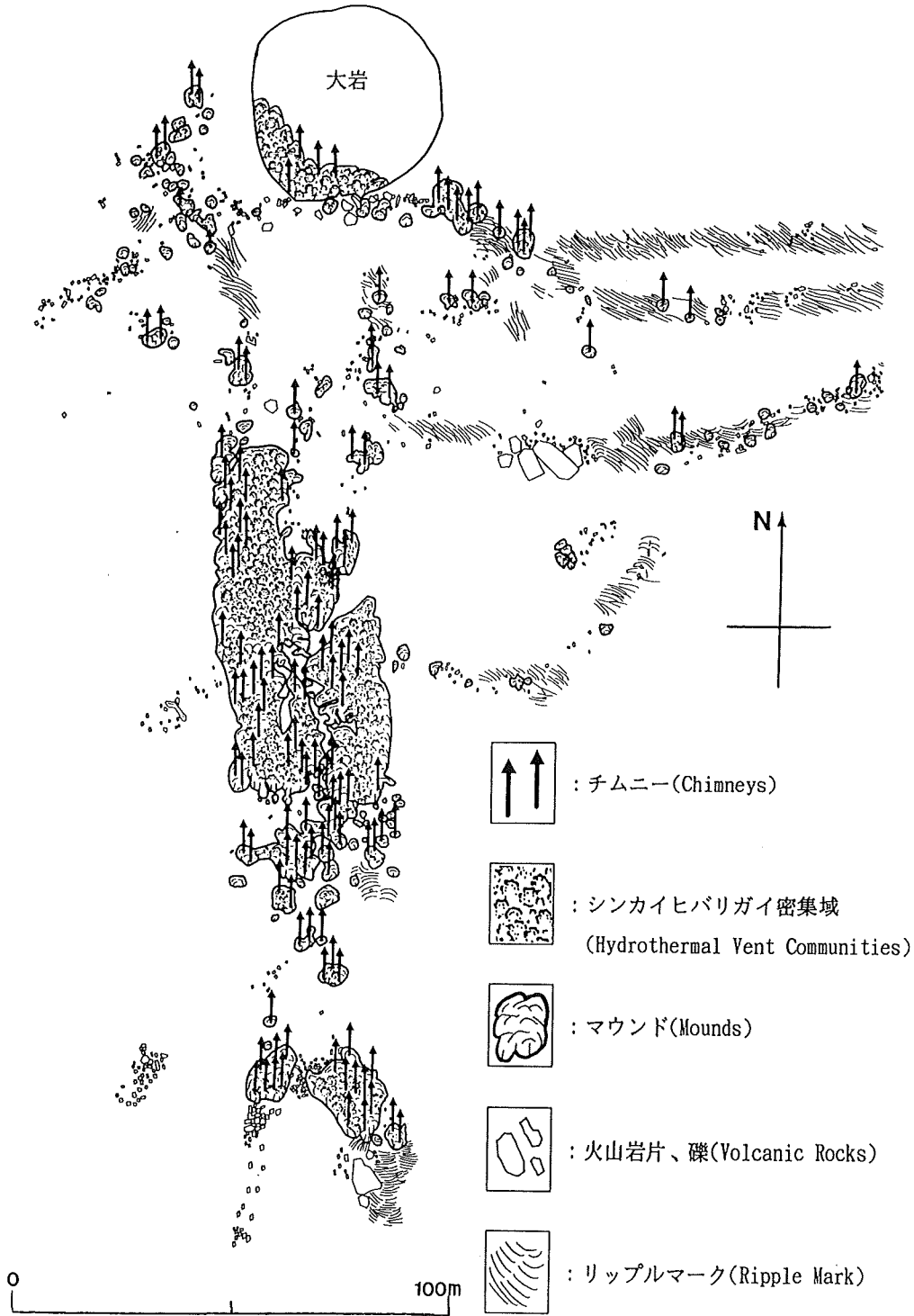
Fig. 42 Hydrothermal activities in the summit crater of the Suiyo Seamount (after Watanabe, in preparation).
