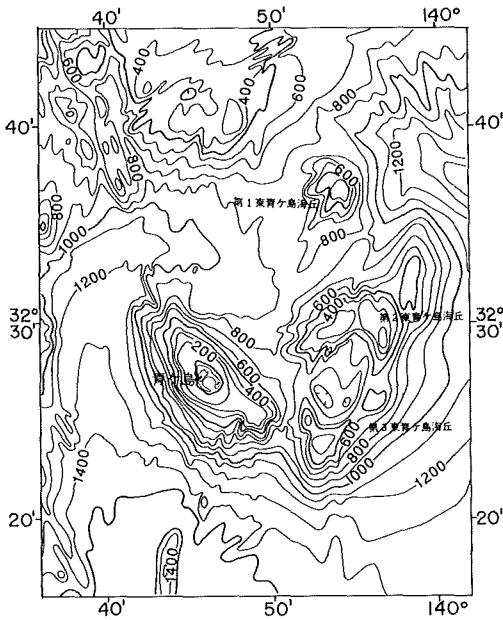
Fig. 33 Topography around Ao-ga-Sima. Surveyed in 1984. Contour interval 100m.
