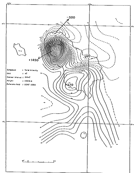
Fig. 32 Aeromagnetic total intensity anomaly chart over Hatizyo Sima volcano at height of 1500m (after Ueda et al. , 1985). Surveyed in 1983. Contour interval 50nT.
