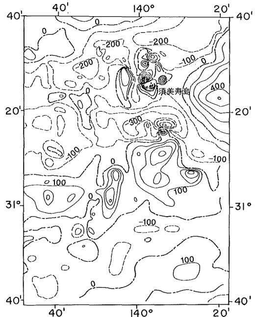
Fig. 38 Geomagnetic total intensity anomaly chart around Sumisu Sima and Daisan-Sumisu Knoll surveyed in 1984. Contour interval 100nT.
