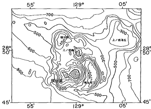
Fig. 12 Topography of Yokoate Sima Volcano surveyed in 1986. Contour interval 100m.
