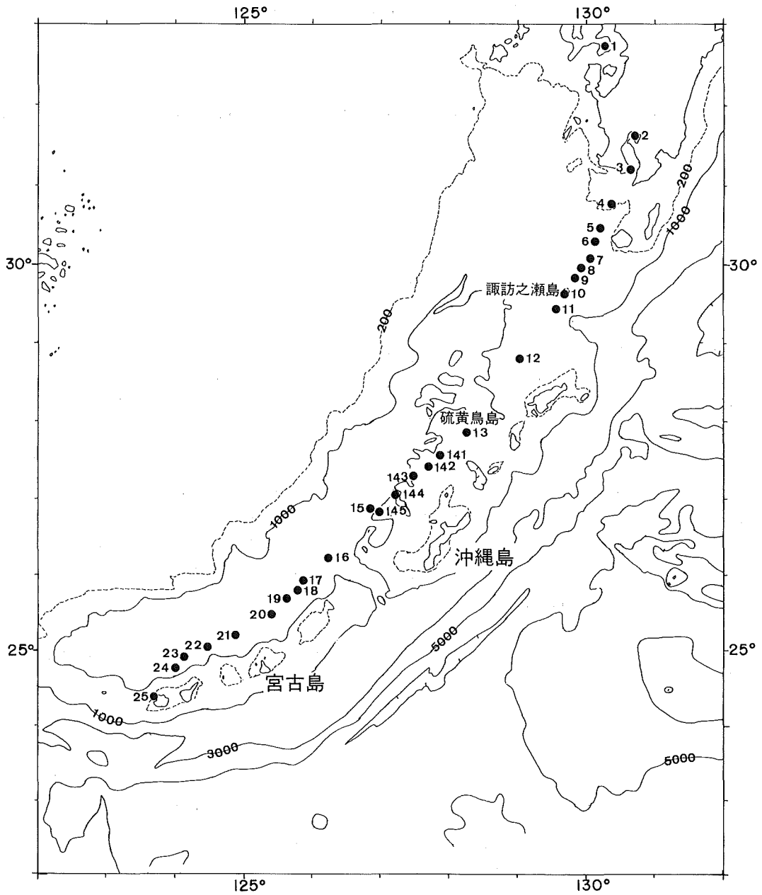
Fig.1 Distribution of volcanoes in the Nansei Syoto Arc. Numbers in the figure refer to each number of volcano listed in this article.
