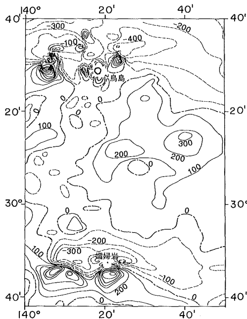
Fig. 40 Geomagnetic total intensity anomaly chart around Tori Sima and Sofu Gan surveyed in 1986. Contour interval 100nT.
