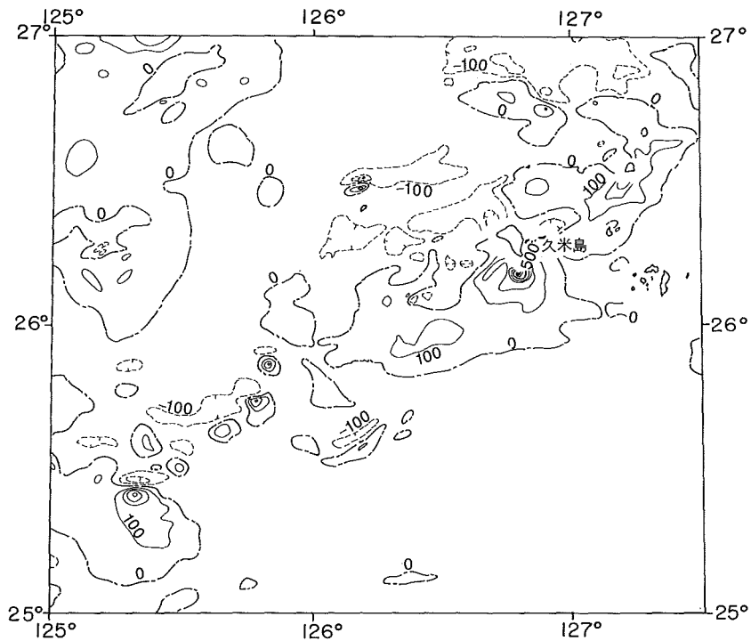
Fig. 15 Geomagnetic total intensity anomaly chart in same area in Fig. 14. Contour interval 100nT.
