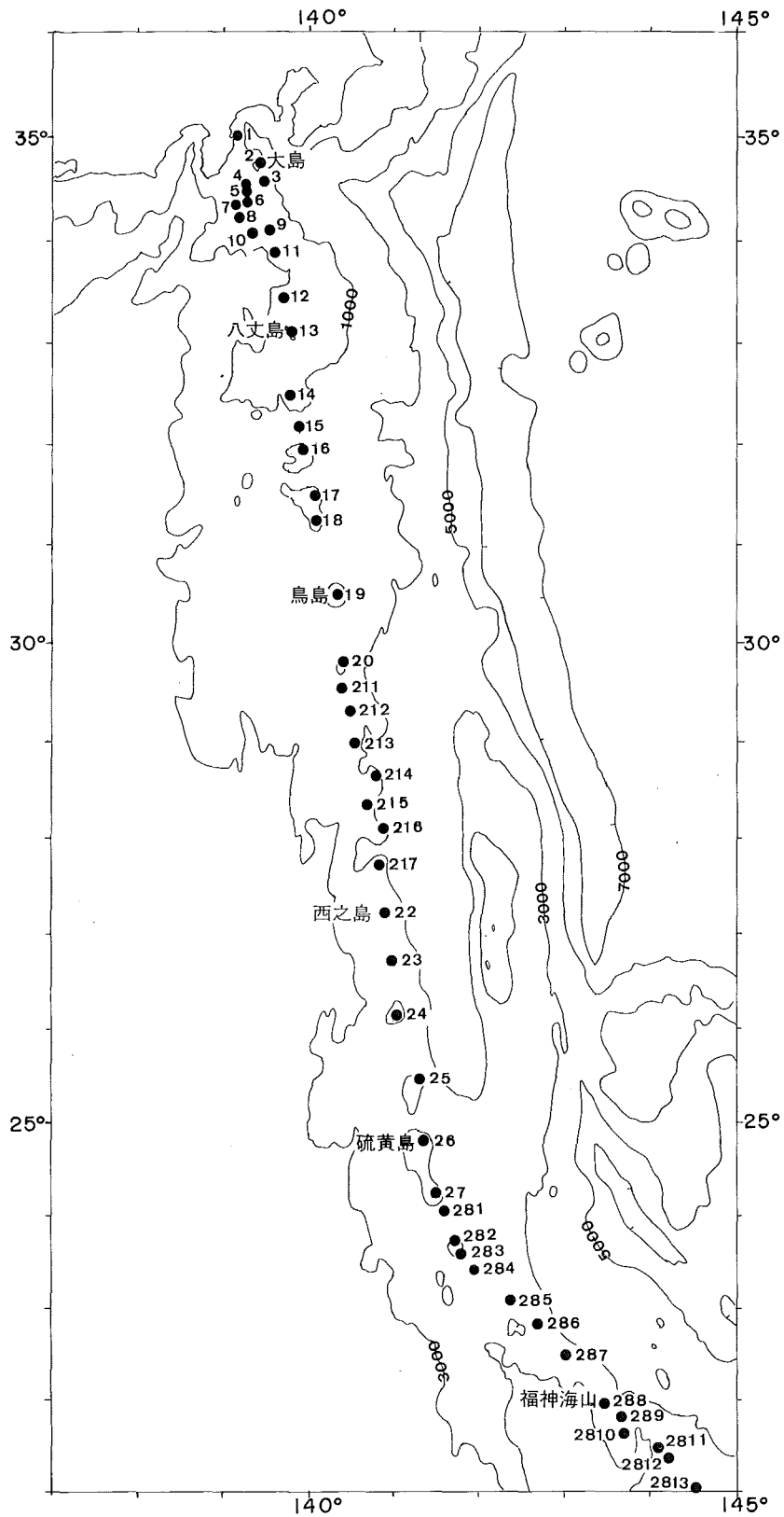
Fig. 2 Distribution of volcanoes in the Nanpo Syoto Arc. Numbers in the figure refer to each number of volcano listed in this article.
