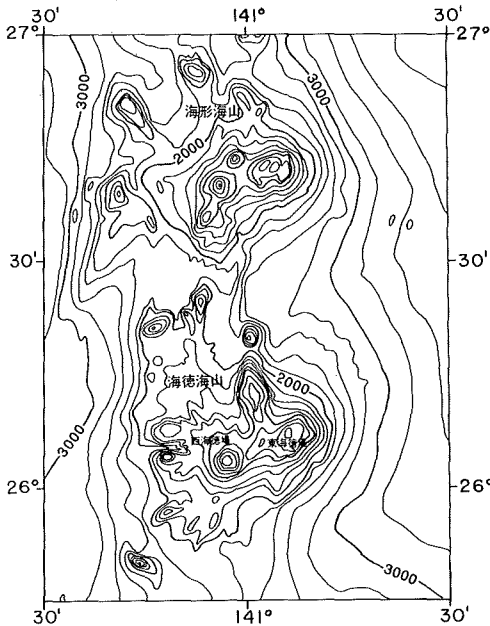
Fig. 45 Topography of Kaikata Seamount and Kaitoku Seamount surveyed on 1985 and 1986. Contour interval 200m.
