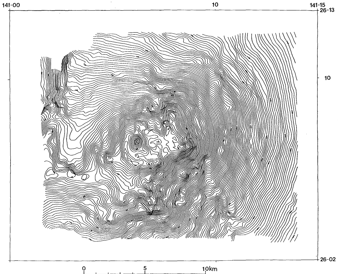
Fig. 47 Topography of Kaitoku Seamount surveyed in 1992. Contour interval 20m.
