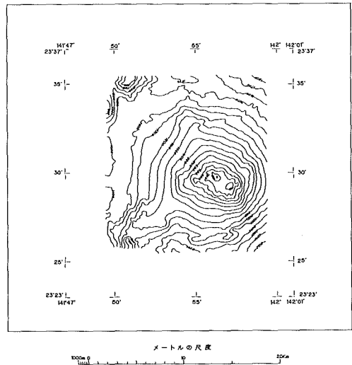
Fig. 53 Topography of Minami-Hiyosi Seamount surveyed in 1990. Contour interval 100m.
