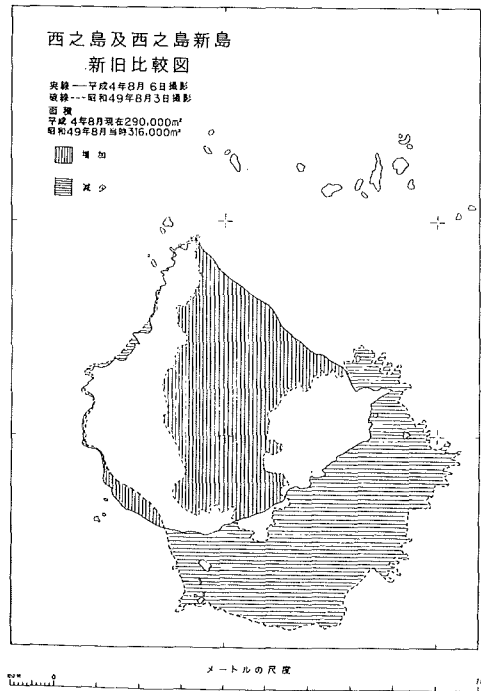
Fig. 44 Nisi-no-Sima and Nisinosima-Sin To in 1974 and 1992. from Report of Coordinating Committee for Prediction of Volcanic Eruption, No.54. (1992)
