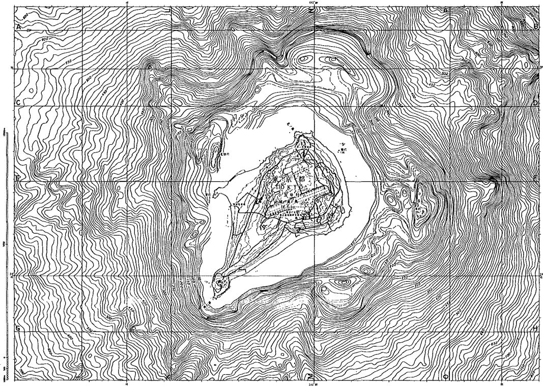
Fig. 49 Topography around Io Sima surveyed in 1991. Contour interval 10m.
