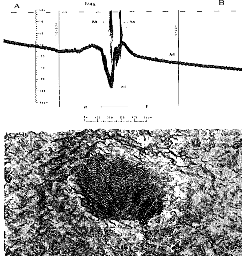
Fig. 20 Echo sounding profile and 3-D image map of the Teisi Knoll from Report of Coordinating Committee for Prediction of Volcanic Eruption, No.45. (1989) A; Echo sounding profile surveyed by "Tenyo" in Oct. 1989, B; 3-D image map viewed from North, in elevation angle : 45°, depth exaggeration : 4 times.
