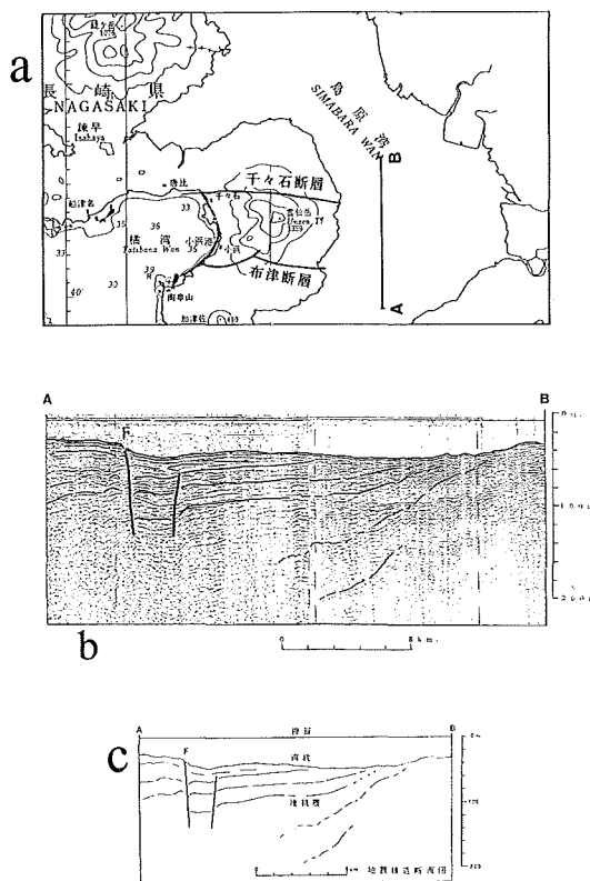
Fig. 3 a; Topography of Unzen volcano. Line A-B shows the seismic profile line. b; Seismic profile along line A-B in Simabara Bay. and c; its line drawing. F shows the fault elongated from Futu Fault. After Hydrog. Dep. Survey Team (1992).
