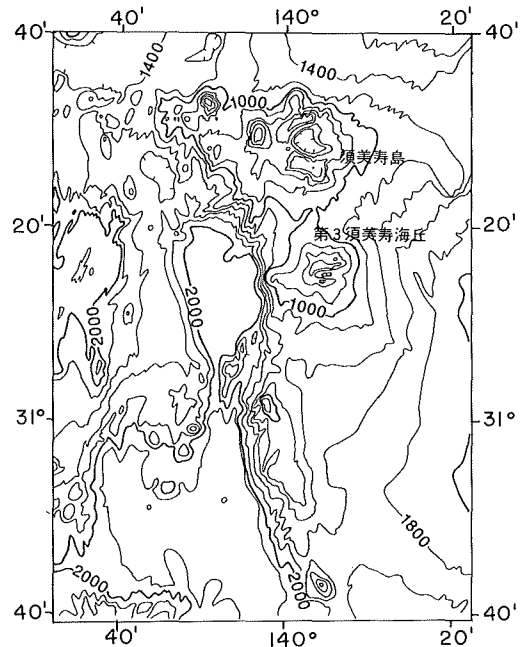
Fig. 37 Topography around Sumisu Sima and Daisan-Sumisu Knoll surveyed in 1984. Contour interval 200m.
