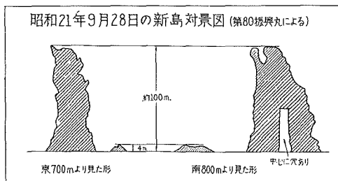
Fig. 36 Sketch of a newly born island at Myozin Syo in 1946 (after Mita, 1949).
