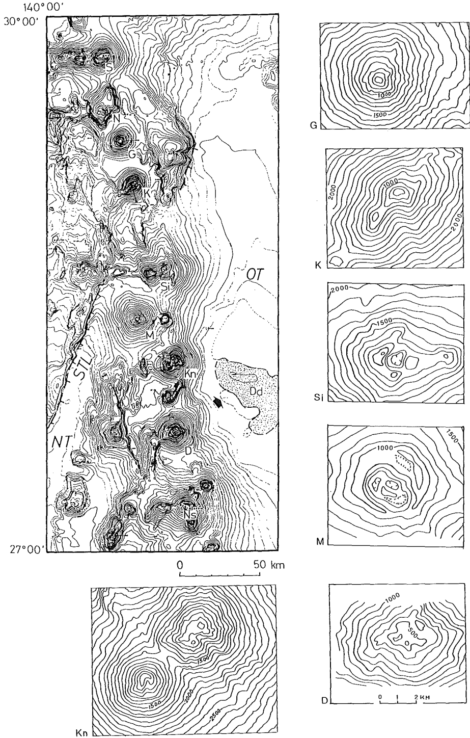
Fig. 41 Topography of Sitiyo Seamount Chain located between Sofu Gan and Nisi-no-Sima and detail topography of the summit of Sitiyo Seamount Chain. S; Sofu gan, N; Nitiyo Seamount, G; Getuyo Seamount, K; Kayo Seamount, Si; Suiyo Seamount, M; Mokuyo Seamount, Kn; Kinyo Seamount, D; Doyo Seamount, Ns; Nisi-no-Sima. Contour interval 100m.
