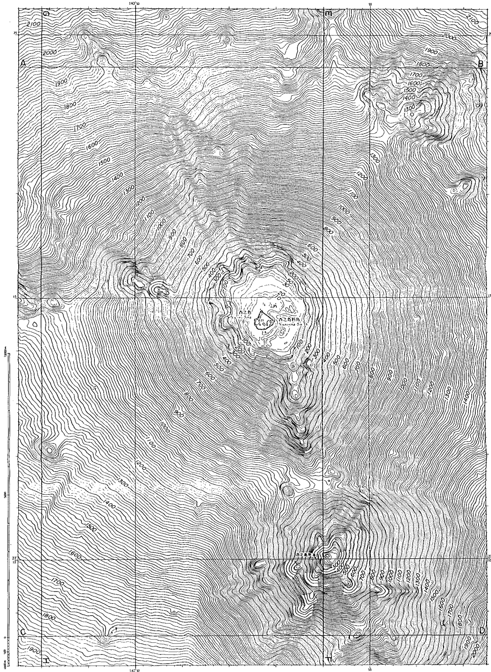
Fig. 43 Topography around Nisi-no-Sima. Contour interval 10m.
