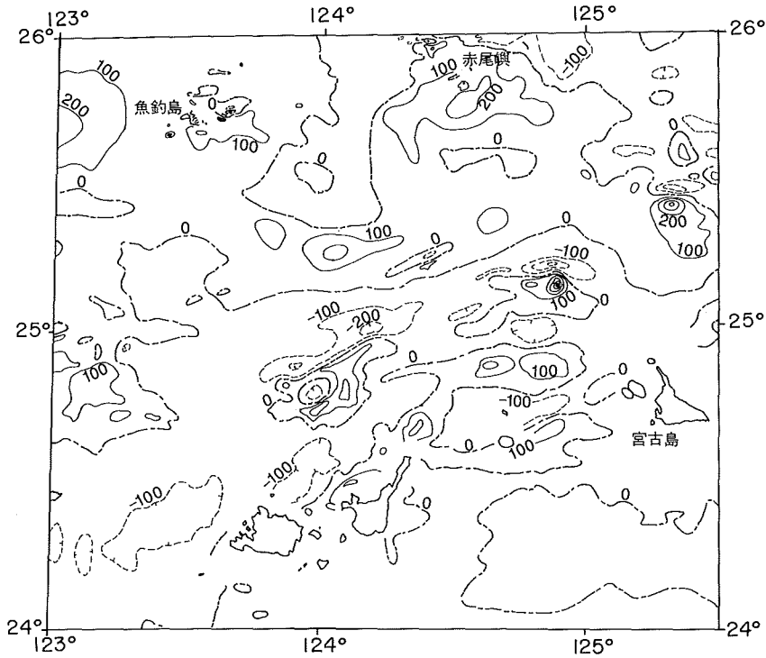
Fig. 17 Geomagnetic total intensity anomaly chart in same area in Fig. 16. Contour interval 100nT.
