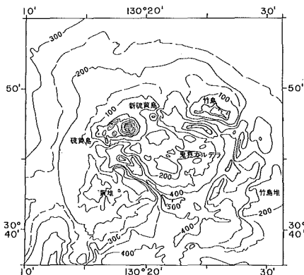
Fig. 9 Topography of Kikai Caldera surveyed in 1980 and 1981. Main contour interval 100m.
