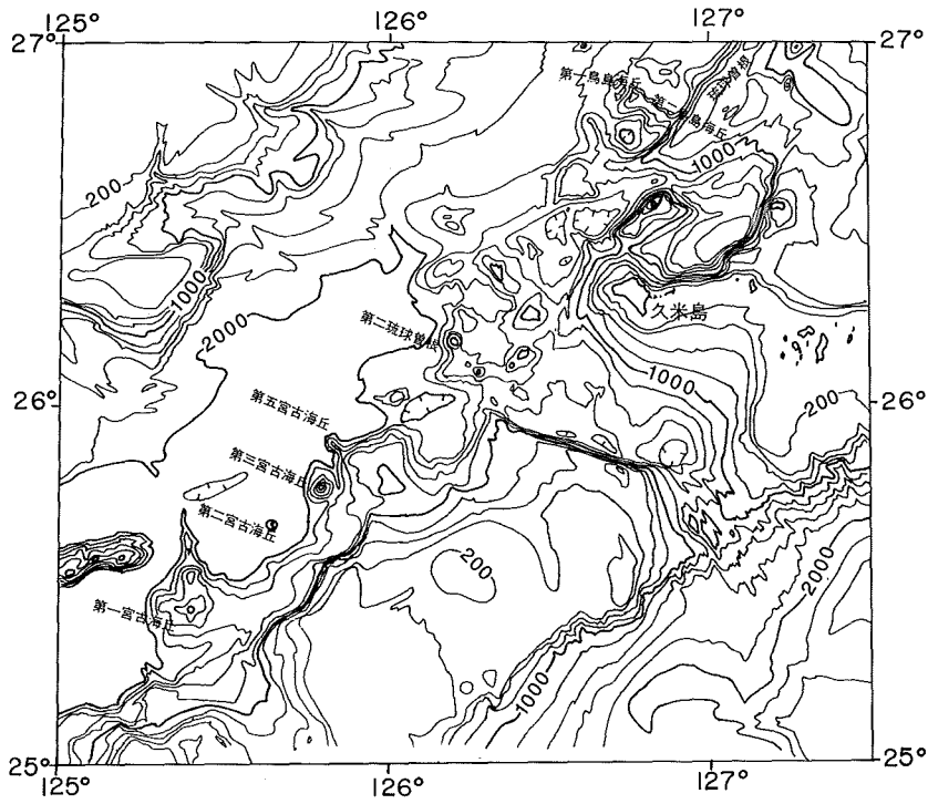
Fig. 14 Topography of volcanic chain in the southern part of the Nansei Syoto arc (Ryukyu Sone to Dai-iti Miyako Knoll) surveyed in 1975, 1976, 1984, 1985 and 1986. Contour interval 200m.
