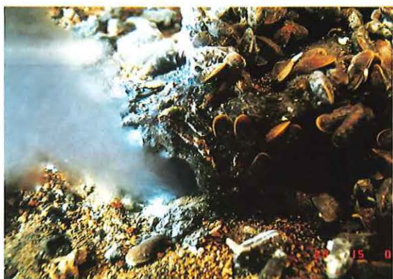
Photo 3 Hydrothermal vent in the summit crater of Suiyo Seamount taken from "Shinkai 2000", JAMSTEC.
