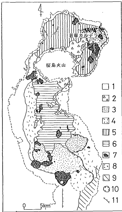
Fig. 8 Geological map of Kagosima Bay from Report of Coordinating Committee for Prediction of Volcanic Eruption, No.46. (1990)
