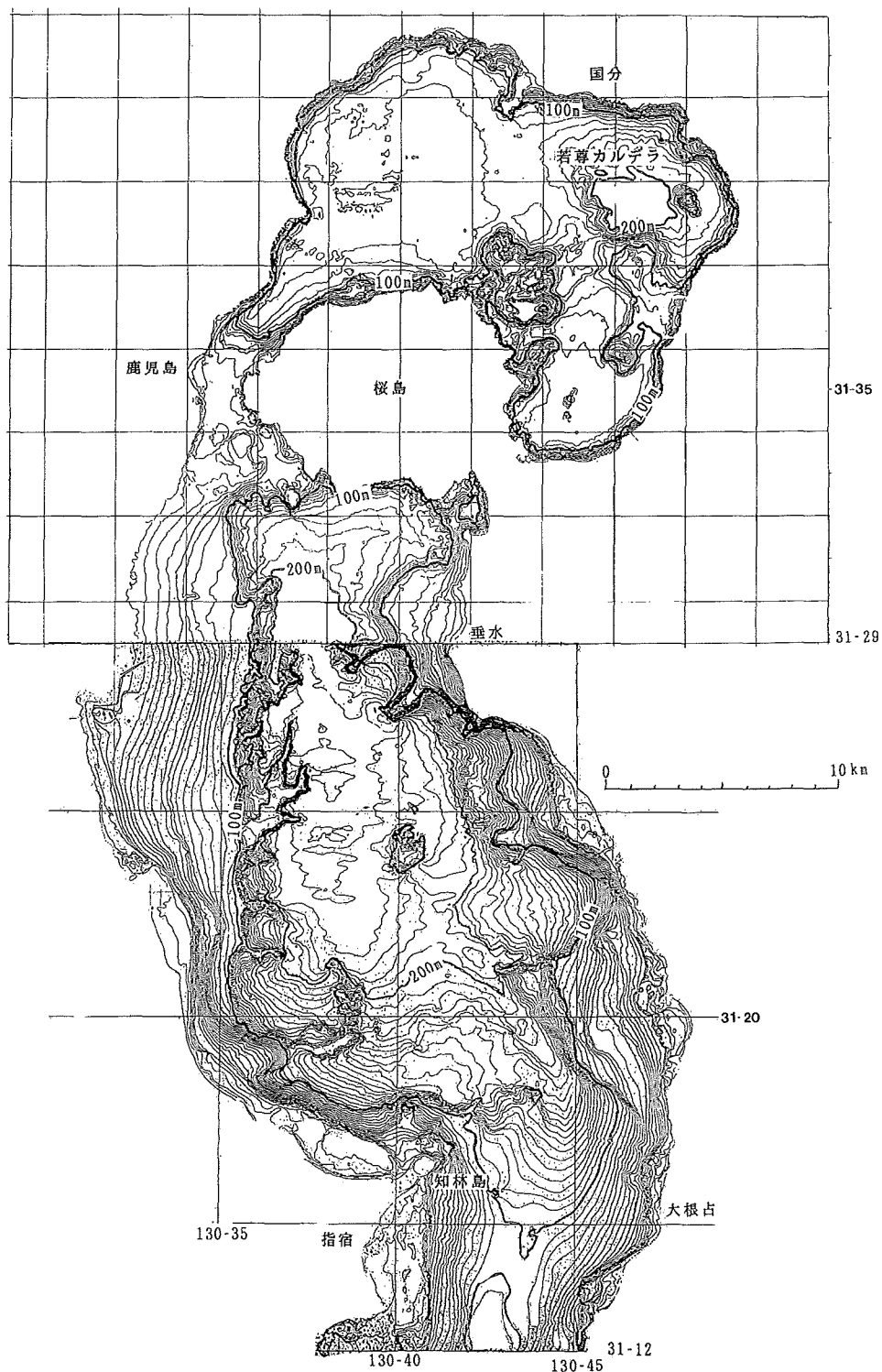
Fig.7 Topography of Kagosima Bay from Report of Coordinating Committee for Prediction of Volcanic Eruption , No.46. (1990)
