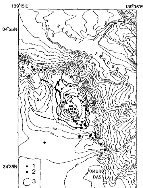
Fig. 21 Topography of Izu-O Sima volcano (after Kato et al. , 1987). Surveyed in 1954, 1974, 1983 and 1986. Contour interval 100m. 1; Flank crater on the island, 2; Knoll, 3; Old volcano.
