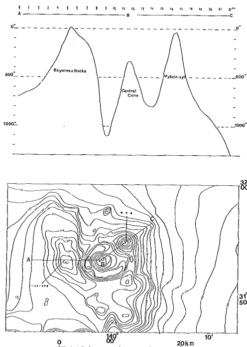
Fig. 35 Topography around Myozin Syo (after Tsukamoto et al. , 1990)
