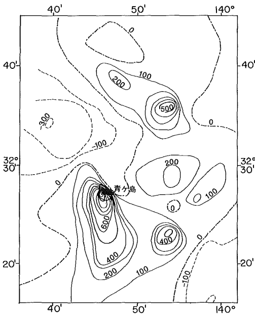
Fig. 34 Aeromagnetic total intensity anomaly chart over Ao-ga-Sima volcano at height of 3000 ft from Report of Coordinating Committee for Prediction of Volcanic Eruption, No.40. (1988) Contour interval 100nT.
