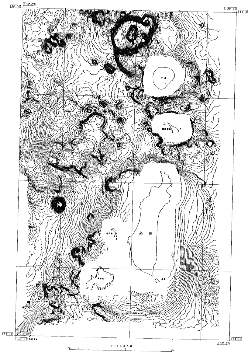
Fig. 23 Topography of Nii Sima surveyed by multibeam sounding system from Report of Coordinating Committee for Prediction of Volcanic Eruption , No. 49. (1991) Contour interval 10m.
