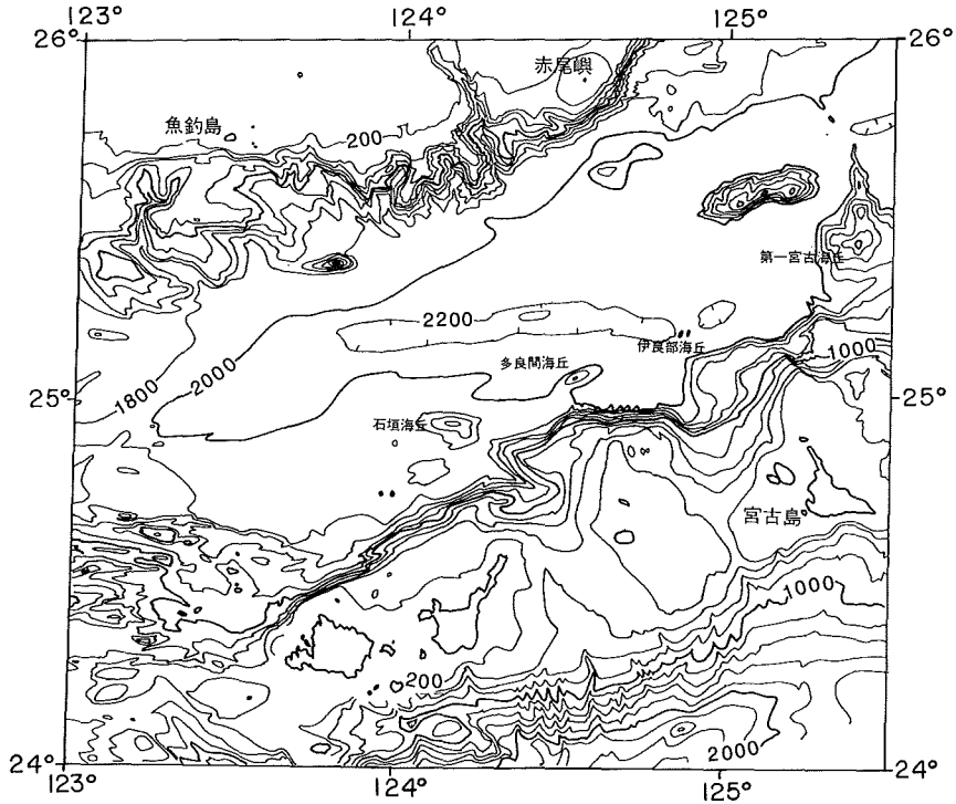
Fig. 16 Topography of volcanic chain in the southern part of the okinawa Trough surveyed in 1976, 1980, 1984 and 1985. Contour interval 200m.
