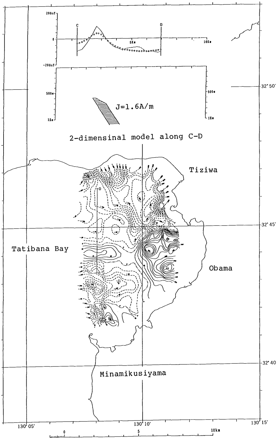
Fig. 5 Geomagnetic total intensity anomaly chart in Tatibana Bay after Hydrog. Dep. Survey Team (1992).
