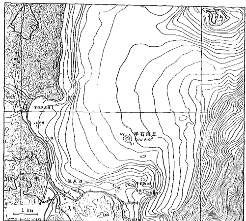
Fig. 18 Topography of Teisi Knoll and its vicinity from Report of Coordinating Committee for Prediction of Volcanic Eruption, No.46, (1990). Contour interval 10m
