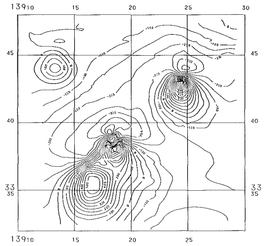
Fig. 30 Geomagnetic total intensity anomaly chart of Mikura Seamount from Report of Coordinating Committee for Prediction of Volcanic Eruption, No51. (1991) Contour interval 50nT.
