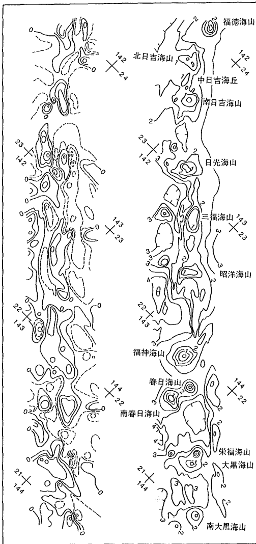
Fig. 52 Chart of topography and magnetic total intensity anomaly in the northern part of the Mariana Ridge surveyed in 1976 and 1977. Right: Topography in interval 500m (until 1000 m); Left: Magnetic anomaly in interval of 100 nT (broken lines show negative).
