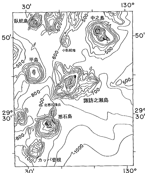
Fig. 11 Topography from Naka-no-Sima to Kappa Sone surveyed in 1974 and 1981. Contour interval 100m.
