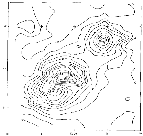
Fig. 31 Free air Gravity anomaly chart of Mikura Seamount from Report of Coordinating Committee for Prediction of Volcanic Eruption, No. 51.(1991) Contour interval 5mGal.
