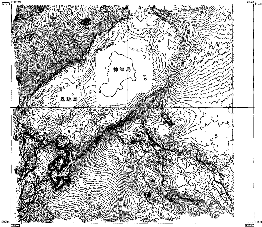
Fig. 25 Topography of Kozu Sima surveyed by multibeam sounding system. Contour interval 10m.
