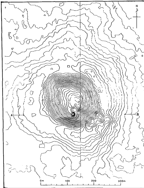
Fig. 19 Detail Topography of Teisi Knoll survey by Hydrochart multibeam sounding system in October 1989 from Report of Coordinating Committee for Prediction of Volcanic Eruption, No.45. (1989) Contour interval 1 m.
