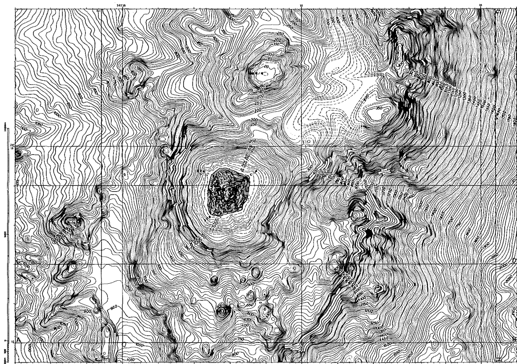
Fig. 51 Topography around Minami-Io Sima surveyed in 1991. Contour interval 10m.
