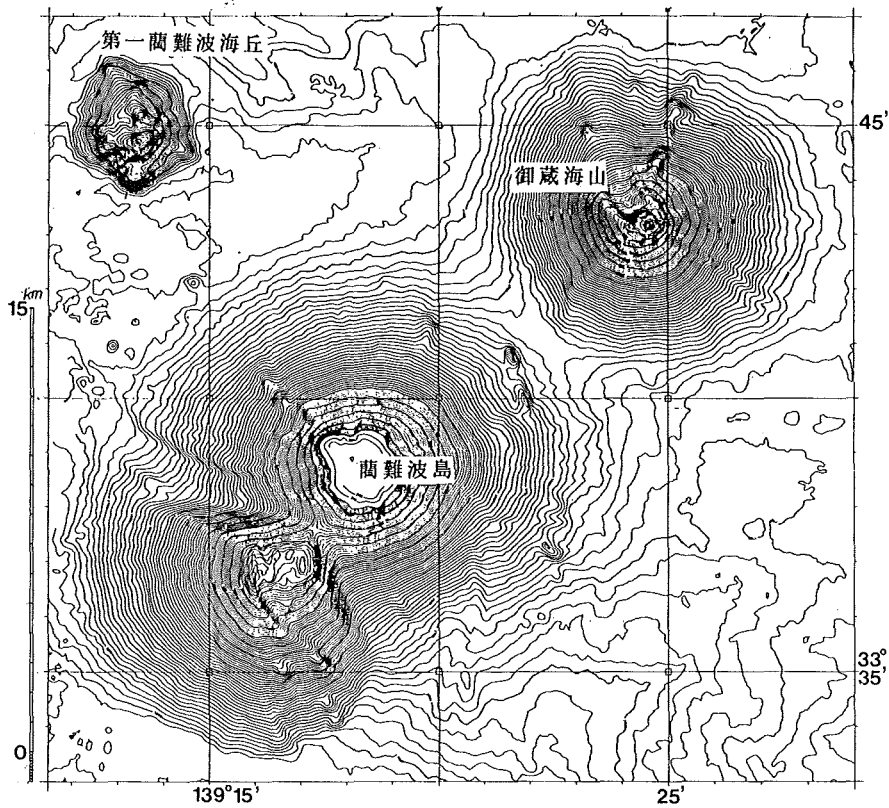
Fig. 29 Topography of Mikura Seamount surveyed by multibeam sounding system from Report of Coordinating Committee for Prediction of Volcanic Eruption , No.51. (1991) Contour interval 1 m.
