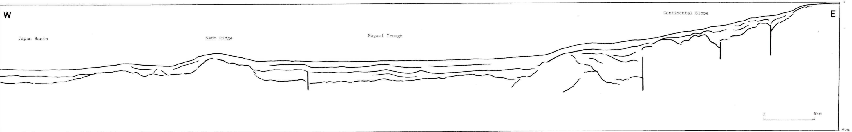
Figure 10 A Migrated depth section (above) and its line drawing (below) of the multi-channel seismic survey by Takuyo.
