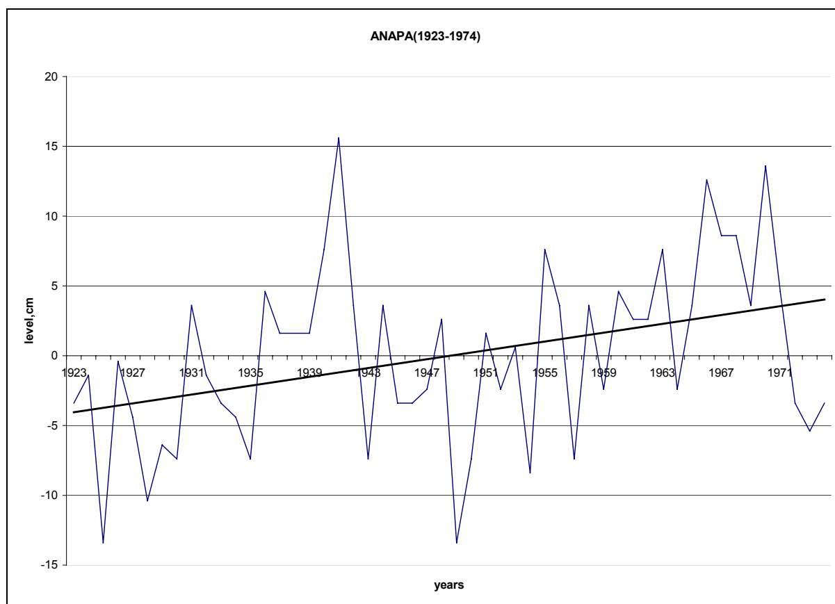
Figure 5. Temporal annual mean sea level variations and linear trend in Anapa (Russia)
