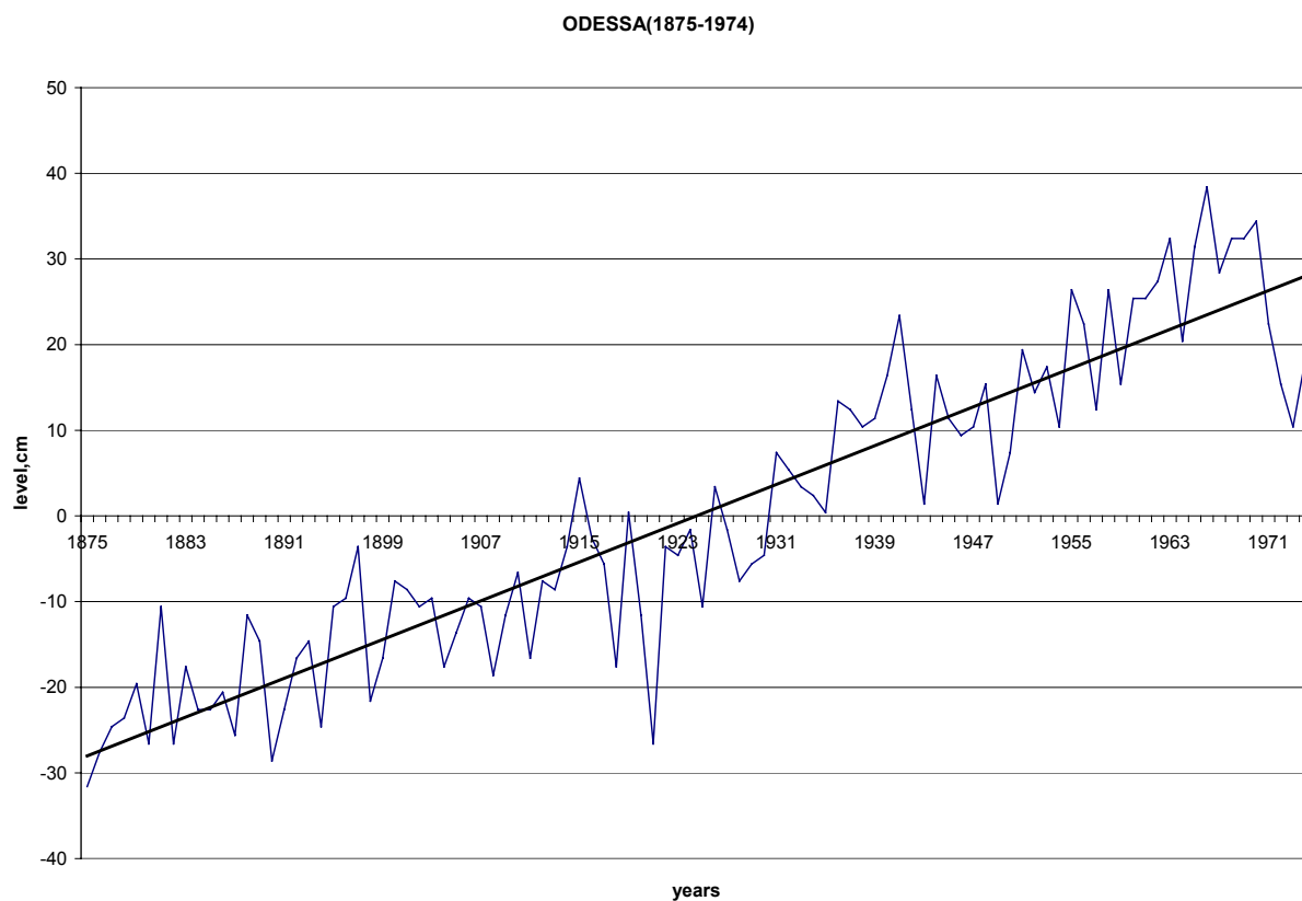
Figure 2. Temporal annual mean sea level variations and linear trend in Odessa (Ukraine)
