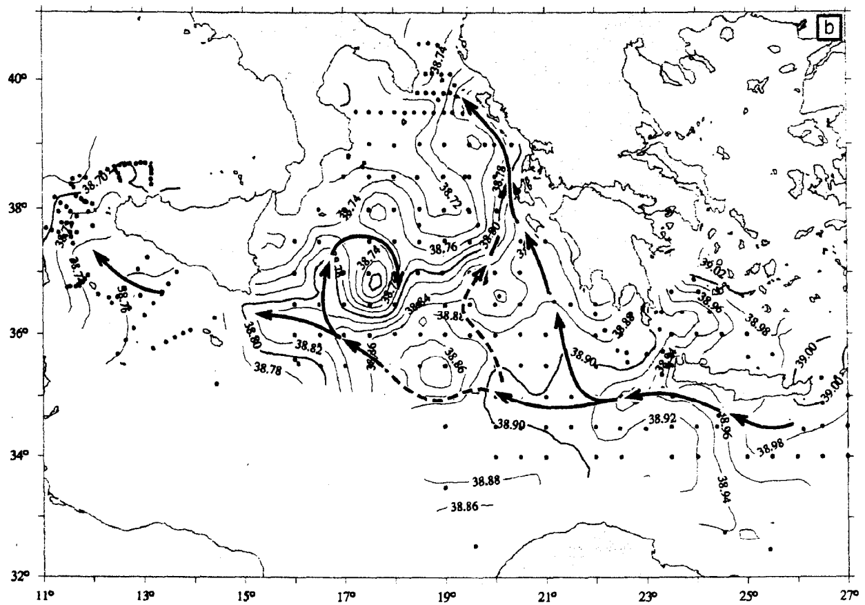
Figure 1 Cruise, POEM-AS87. Salinity at density = 29.05 \text{ kg/m}^3
