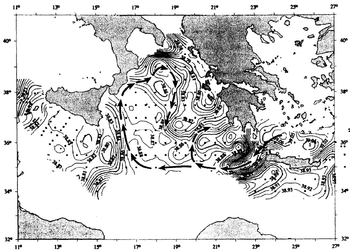
Figure 3 Cruise, POEMBC-091. Salinity at density = 29.10 kg/m 3
