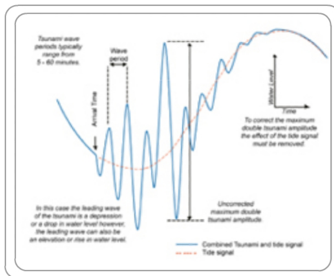
Mareogram (sea level) record of a tsunami.
