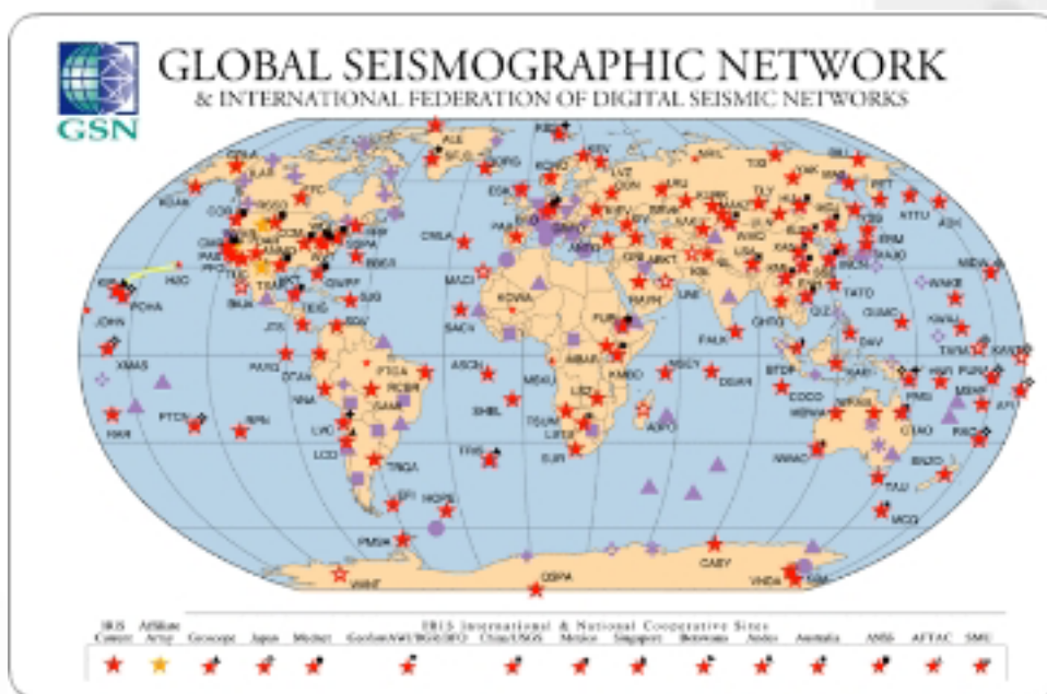
Global Seismographic Network
