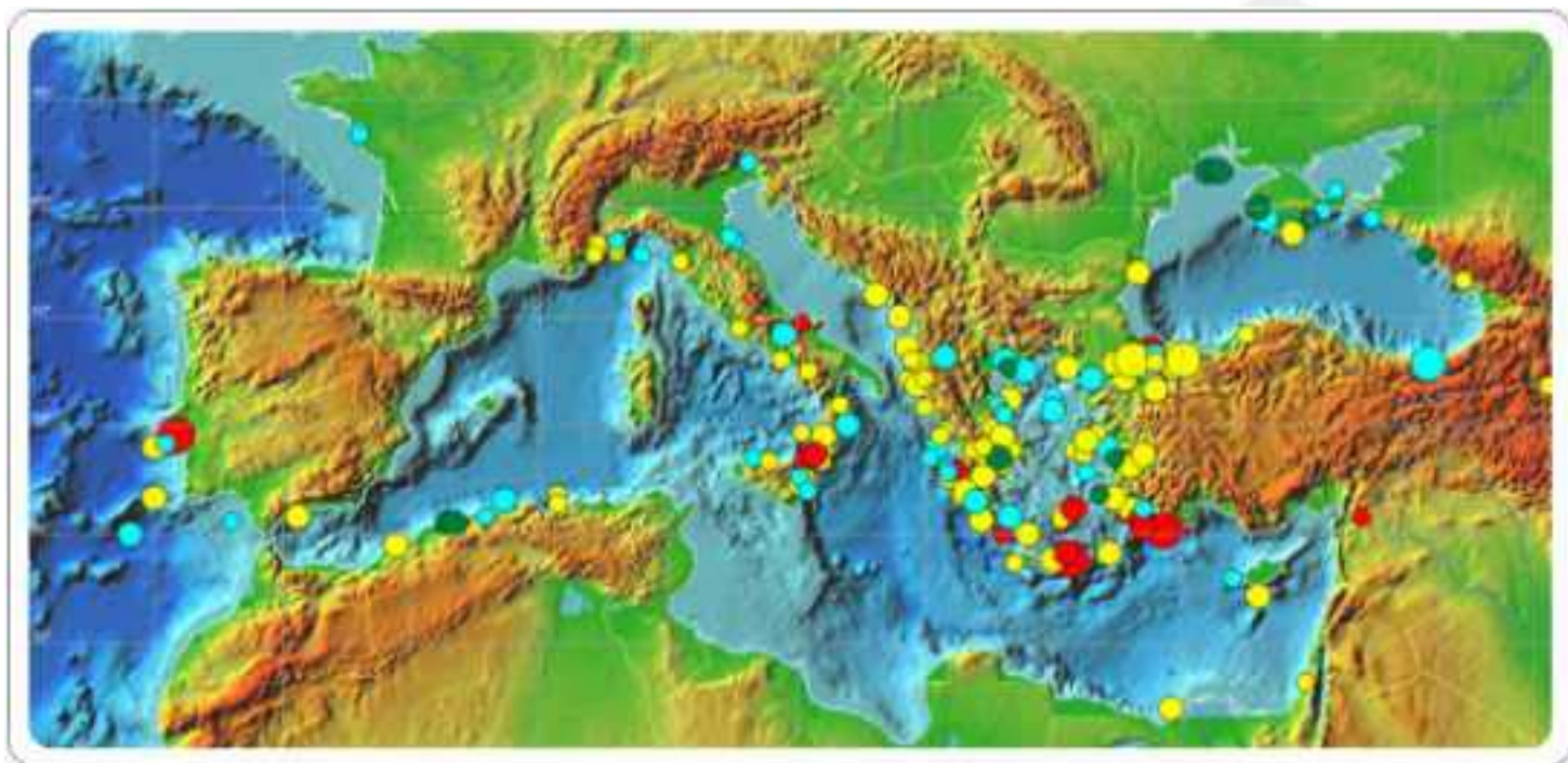
Earthquakes generating tsunamis in the Mediterranean and connected seas. Circle color indicates extent of tsunami damage (greatest is red, followed by yellow, blue, and green). The size of the circle is scaled to the magnitude of the earthquake. Source: ITDB, 2005.
