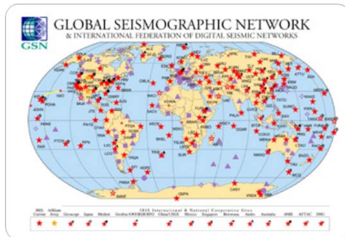
Global Seismographic Network
