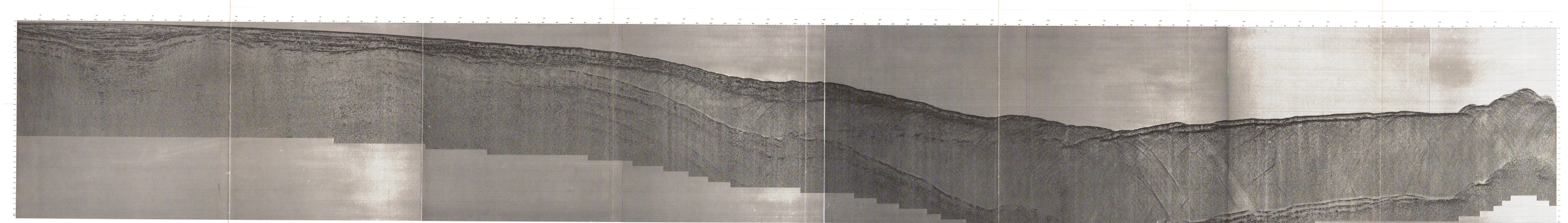
Figure 3 Multichannel seismic reflection profile of 24 fold record section off Joban District, Northeast-Japan abscissa: 500 meters/division, ordinate: 0.1 seconds/division (two-way) vertical exaggeration : 2.5 (at sea bottom)
