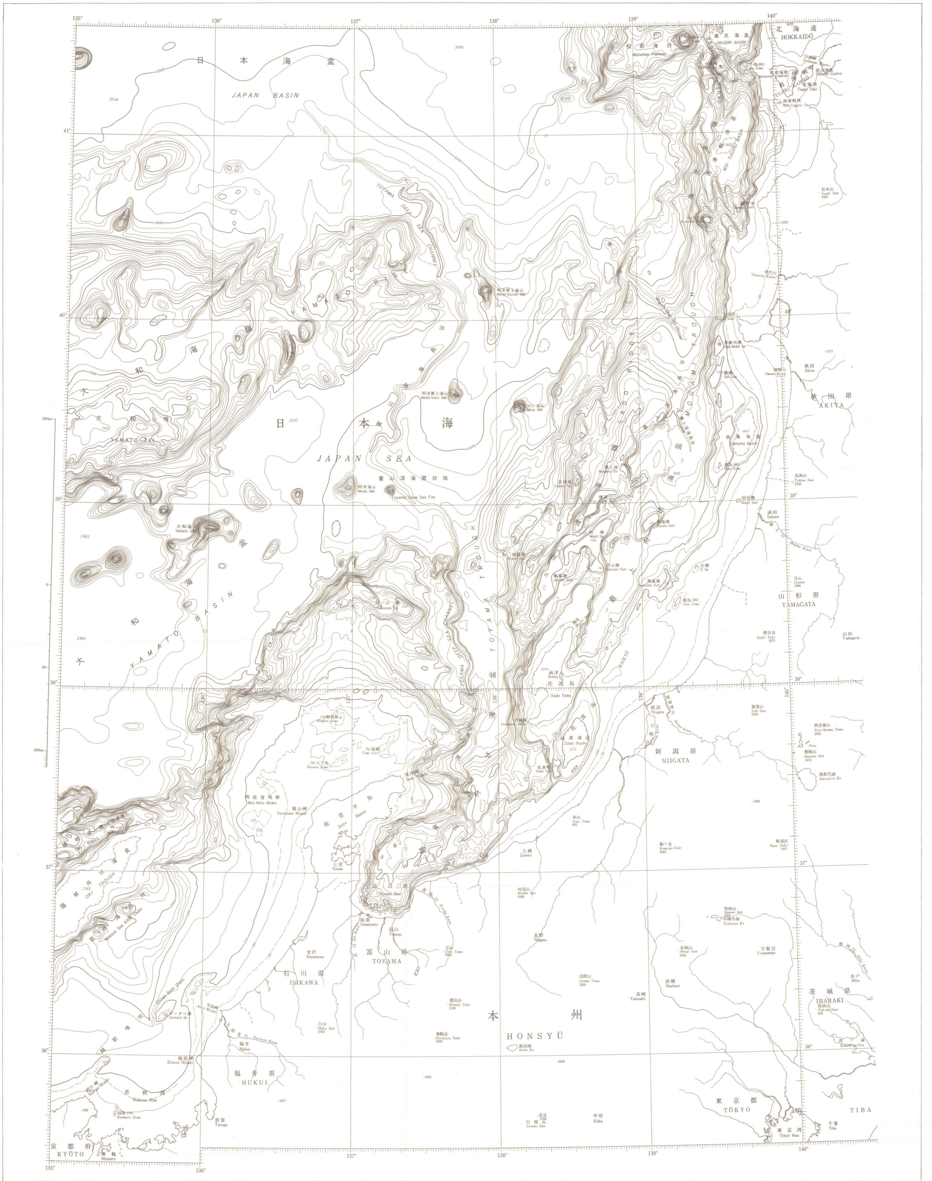
Figure 5. Bathymetric chart, Westward of Tohoku.
