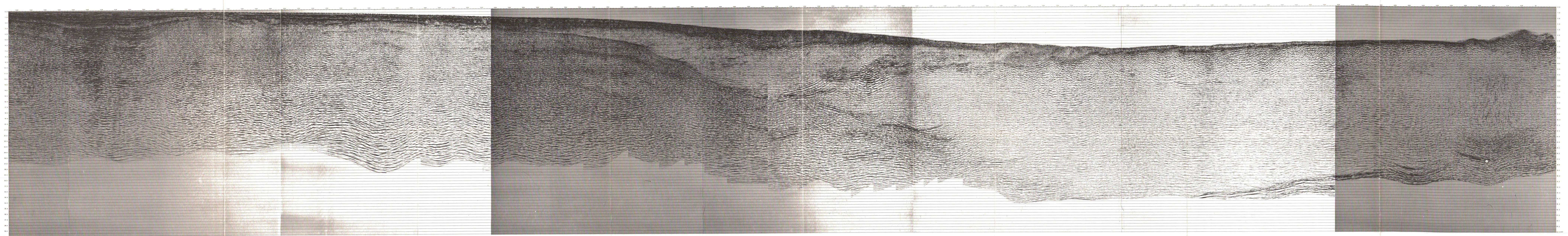
Figure 5 Multichannel seismic reflection profile of migrated depth section off Joban District, Northeast-Japan abscissa: 500 meters/division, ordinate: 500 meters/division vertical exaggeration : 1
